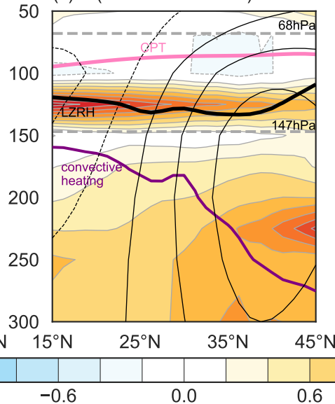
(c) \theta (MERRA-2-MRM)
