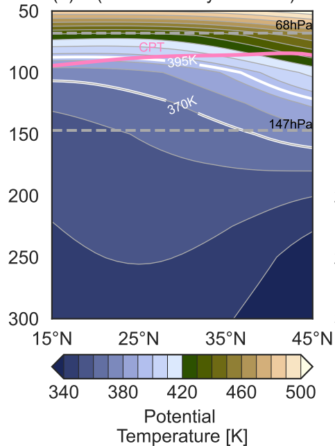
(a) \theta (Multi-Reanalysis Mean)
