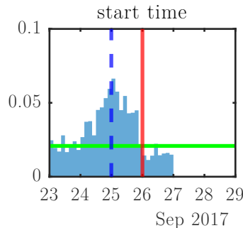
wet deposition
