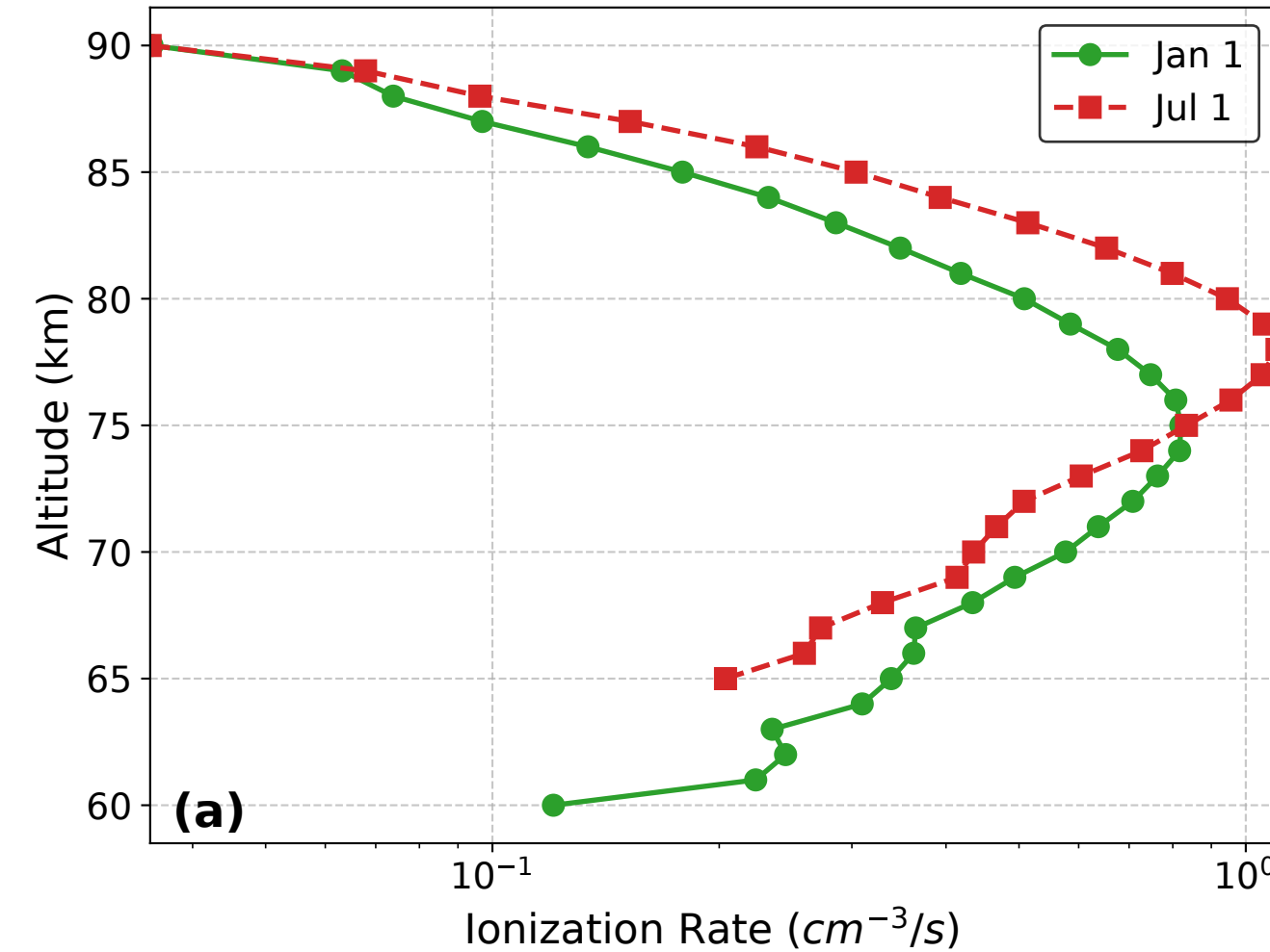
Ionization Rate q
