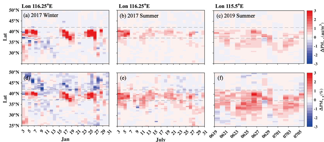
Figure 9. Simulated responses of daily average (daytime) \text{PM}_{2.5} to observational constraints on aerosol vertical distribution along the longitude profiles of observation stations. (a–c) Mass concentration ( \mu\text{g m}^{-3} ) and (d–f) proportion (%). From left to right: for winter 2017 (a, d), summer 2017 (b, e), and summer 2019 (c, f), respectively. The dotted lines indicate the latitude range of the modified region, and the longitudes of the stations are marked at the top.
