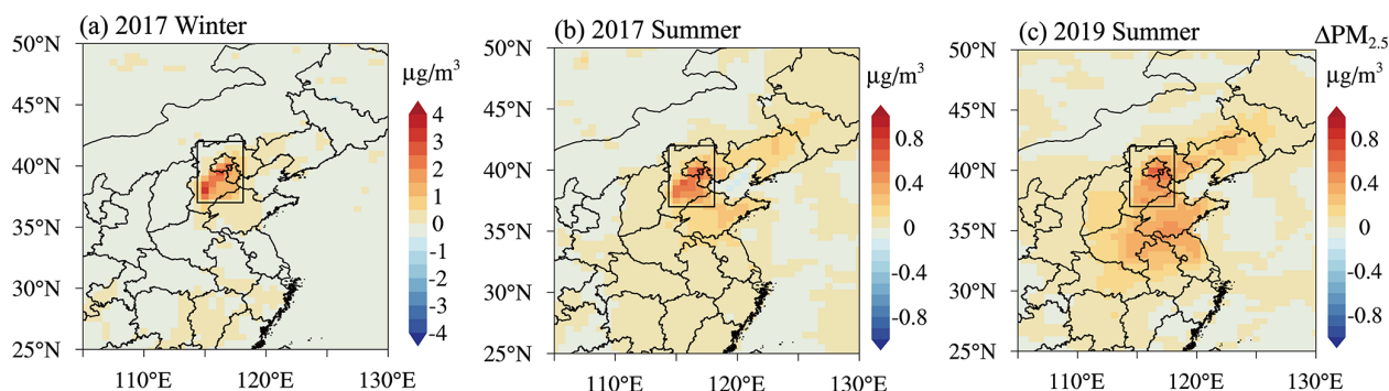
Figure 8. Simulated responses of \text{PM}_{2.5} concentration to observational constraints on aerosol vertical distribution over North China. From left to right: winter 2017 (a), summer 2017 (b), and summer 2019 (c), respectively. The black rectangle shows the region where vertical distribution modification was performed.
