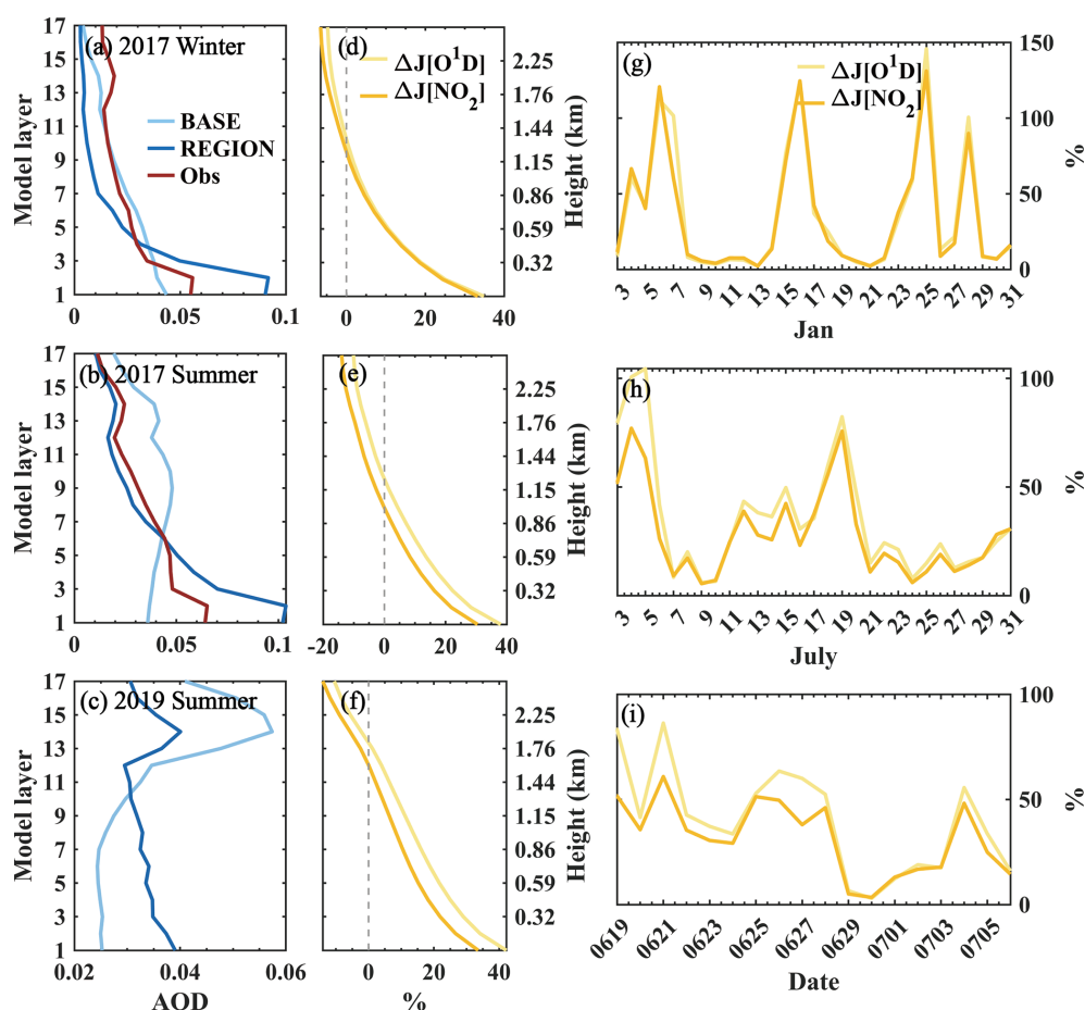
Figure 2. Vertical profiles of average (a–c) AOD and (d–f) relative changes of J[\text{NO}_2] , and J[\text{O}^1\text{D}] in model layers at observation stations. The red, light, and dark blue lines represent observed, BASE-simulated, and REGION-simulated AOD, respectively. (g–i) Time series of daily average relative changes of surface J[\text{NO}_2] and J[\text{O}^1\text{D}] at observation stations. From top to bottom: winter 2017 (a, d, g), summer 2017 (b, e, h), and summer 2019 (c, f, i), respectively. The averages are calculated using data during the daytime when photolysis occurs.
