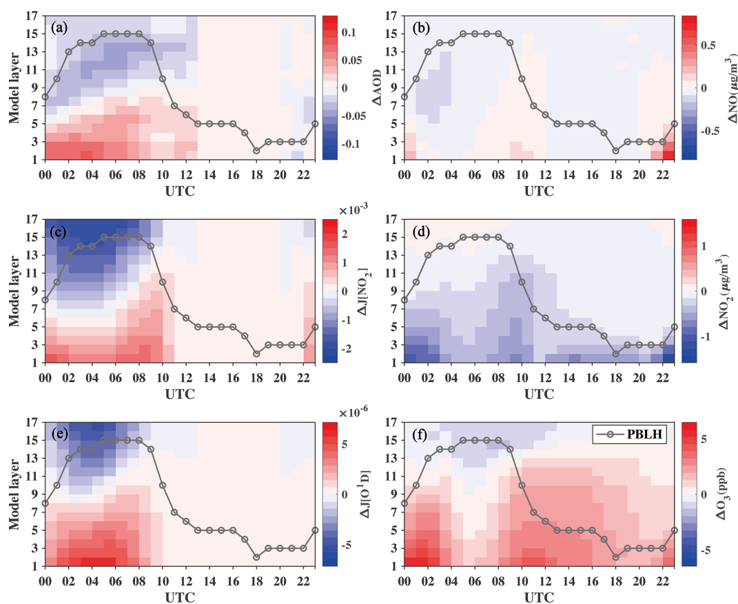
Figure 6. Diurnal variation in the vertical distribution responses of (a) AOD, (c) J[\text{NO}_2] , (e) J[\text{O}^1\text{D}] , (b) nitric oxide (NO), (d) nitrogen dioxide ( \text{NO}_2 ), and (f) ozone at the observation stations under conditions with high planetary boundary layer height (PBLH).
