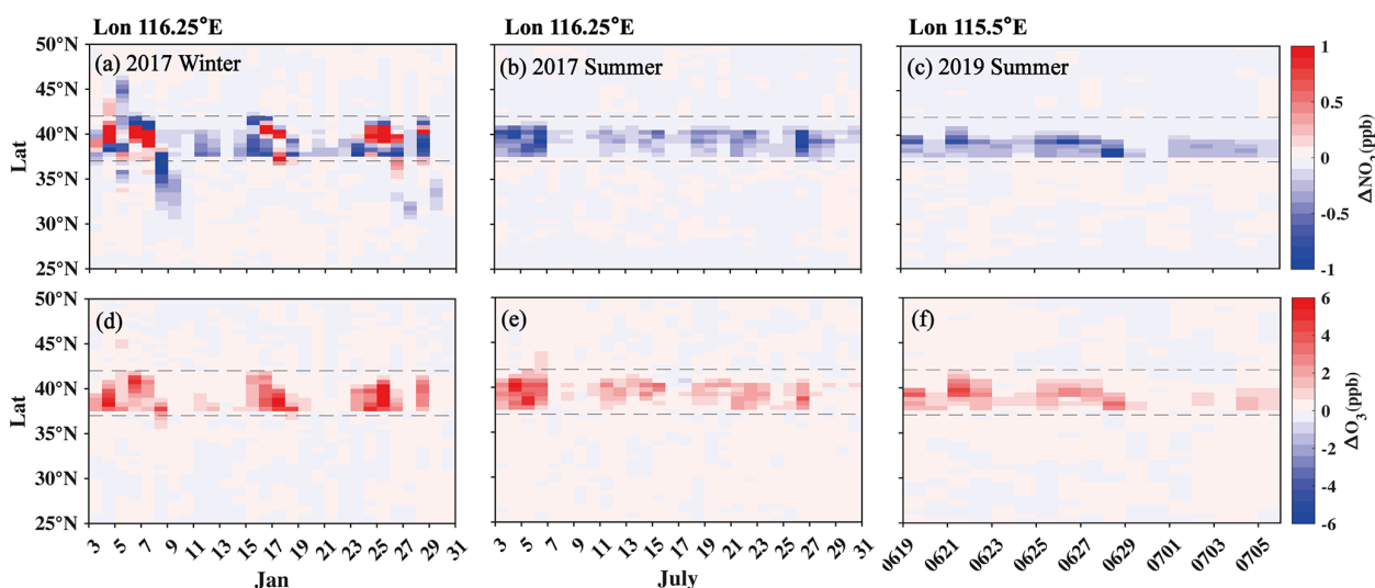
Figure 5. Simulated responses of daytime average ozone and nitrogen dioxide (NO 2 ) to observational constraints on aerosol vertical distribution along the longitude profiles of observation stations. From left to right: winter 2017 ( a , d ), summer 2017 ( b , e ), and summer 2019 ( c , f ), respectively. The dotted lines indicate the latitude range of the modified region, and the longitudes of the stations are marked at the top.
