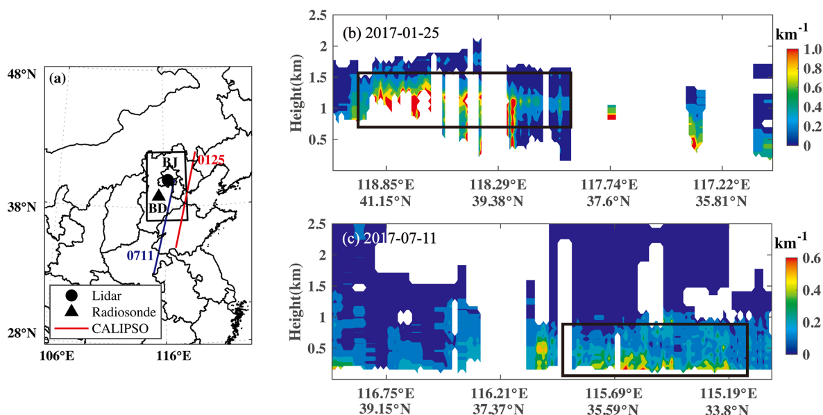
Figure 1. (a) Spatial distribution of lidar and radiosonde stations. BJ: Beijing; BD: Baoding. The black rectangle shows the region where vertical distribution modification was performed. Vertical distribution of aerosol extinction coefficient (532 nm) from CALIPSO on (b) 25 January 2017 and (c) 11 July 2017. The corresponding CALIPSO overpassing tracks are marked with red and blue lines in (a).
