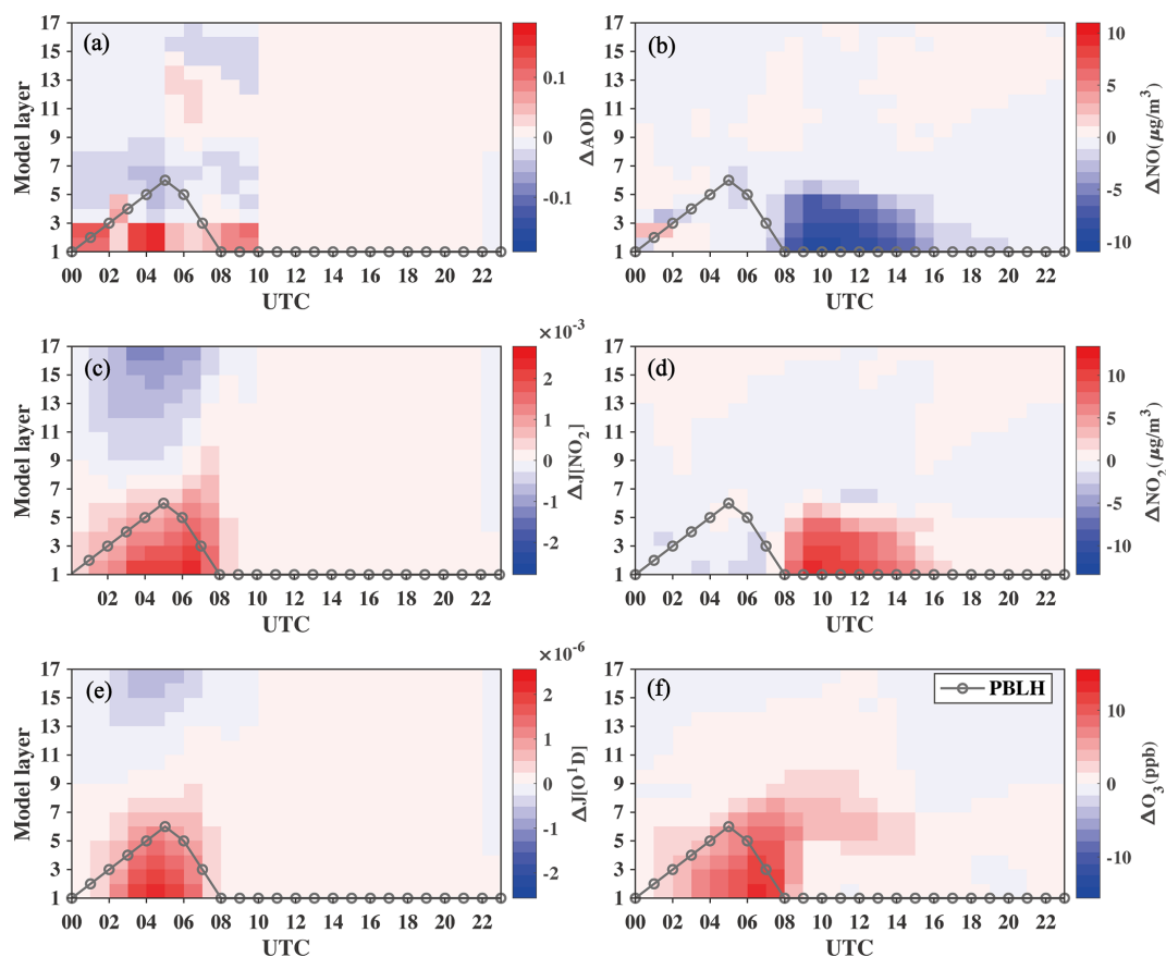
Figure 7. Same as Fig. 6 but under conditions with lower planetary boundary layer heights (PBLHs).
