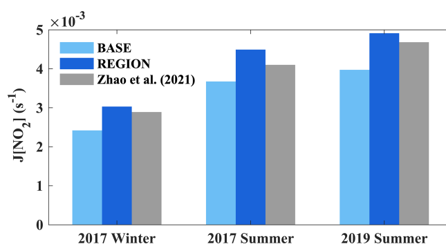
Figure 3. Simulated and observed average surface J[\text{NO}_2] at Xianghe station for winter 2017, summer 2017, and summer 2019. The seasonal average J[\text{NO}_2] from Zhao et al. (2021) is presented by grey bars.
