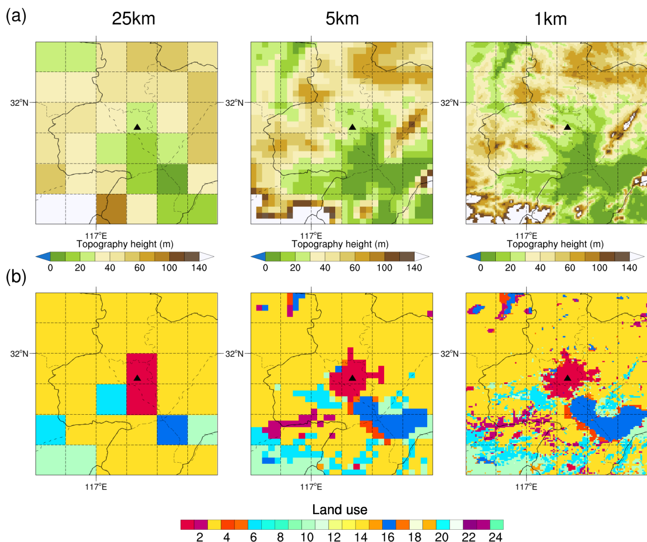
Figure 1. (a) The terrain height (m) in the study area for simulations with respective resolutions of 25 km (left), 5 km (middle), and 1 km (right). (b) Spatial distribution of land use types in the study area for simulations with respective resolutions of 25 km (left), 5 km (middle), and 1 km (right). The solid black triangle indicates the location of the USTC site.
