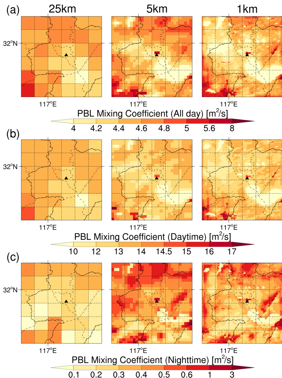
Figure 10. Spatial distribution of PBL mixing coefficients in the study area for (left) 25 km, (middle) 5 km, and (right) 1 km resolution simulations of (a) the whole day, (b) daytime, and (c) nighttime, respectively. The solid black triangle indicates the location of the USTC site. The simulation results are from the three sensitivity experiments.
