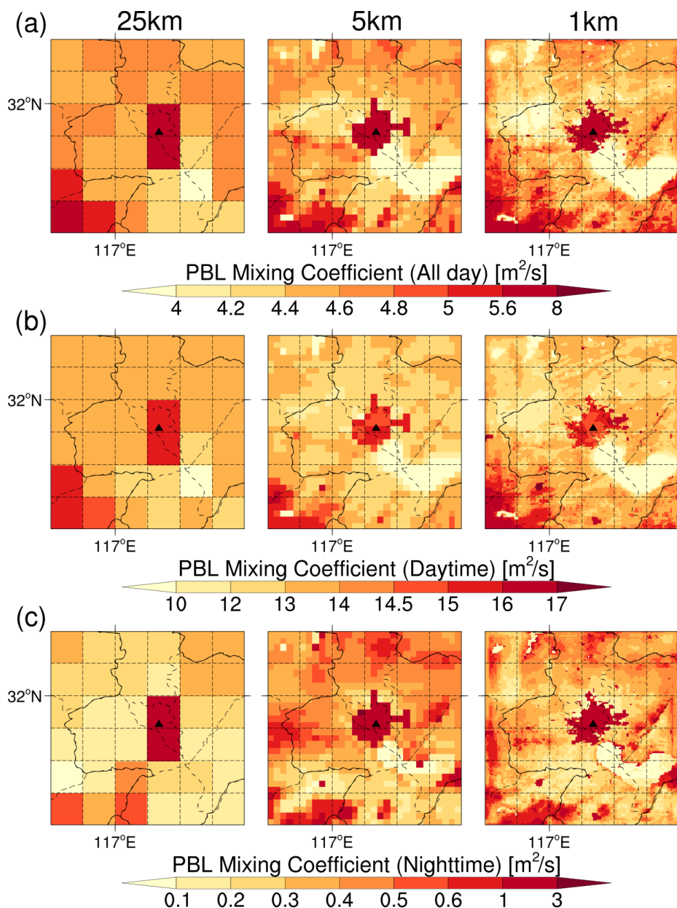
Figure 7. Spatial distribution of PBL mixing coefficients in the study area for 25 km (left), 5 km (middle), and 1 km (right) resolution simulations of (a) the whole day, (b) daytime, and (c) nighttime, respectively. The solid black triangle indicates the location of the USTC site.
