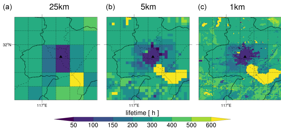
Figure 13. Spatial distribution of the BC lifetime in the study area for (a) 25 km, (b) 5 km, and (c) 1 km resolution simulations of the whole day, respectively. The solid black triangle indicates the location of the USTC site.
