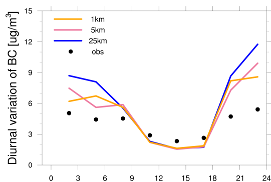
Figure 5. Diurnal variation in BC surface concentrations within 24 h averaged over the USTC site during the study period for 25 km (solid blue line), 5 km (solid pink line), and 1 km (solid orange line) resolution simulations and observations (black dot). Both the simulated results and observations are sampled at the model output frequency, i.e., 3 h.
