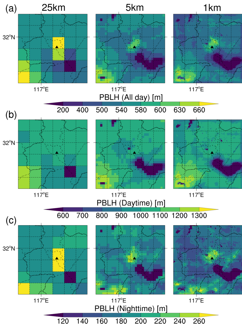
Figure 6. Spatial distribution of the PBL height in the study area for 25 km (left), 5 km (middle), and 1 km (right) resolution simulations of (a) the whole day, (b) daytime, and (c) nighttime, respectively. The solid black triangle indicates the location of the USTC site.
