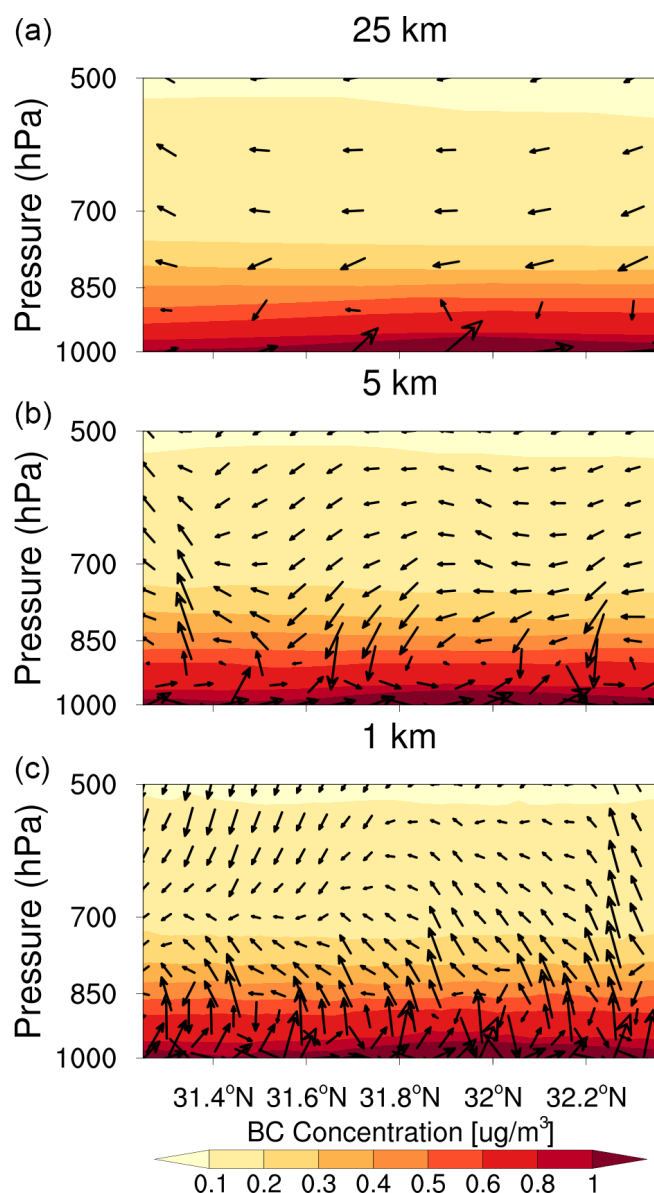
Figure 8. The latitude–pressure cross section of BC concentrations and wind speed flux along the USTC site for 25 km (a), 5 km (b), and 1 km (c) resolution simulations of the whole day. Vector arrows are the combination of wind speed fluxes v and w , with the vertical wind speed flux being multiplied by 100 for visibility. The shaded contours represent BC concentrations at each pressure level.
