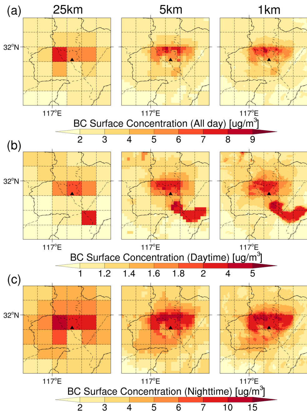
Figure 4. Spatial distribution of the BC surface concentration in the study area for 25 km (left), 5 km (middle), and 1 km (right) resolution simulations of (a) the whole day, (b) daytime, and (c) nighttime, respectively. The solid black triangle indicates the location of the USTC site.
