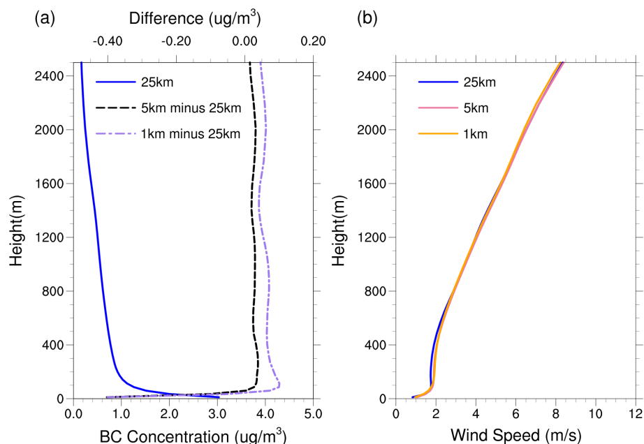
Figure 12. (a) Vertical profiles of BC concentrations simulated at a 25 km resolution (solid blue line), the difference between resolutions of 5 and 25 km (dashed black line), and the difference between resolutions of 1 and 25 km (dashed purple line) averaged over the study area for the whole day, respectively. (b) Vertical profiles of wind speed simulated at a 25 km resolution (solid blue line), 5 km resolution (solid pink line), and 1 km resolution (solid orange line) averaged over the study area for the whole day, respectively.
