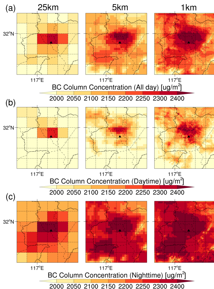
Figure 11. Spatial distribution of the BC column concentration in the study area for (left) 25 km, (middle) 5 km, and (right) 1 km resolution simulations of (a) the whole day, (b) daytime, and (c) nighttime, respectively. The solid black triangle indicates the location of the USTC site.
