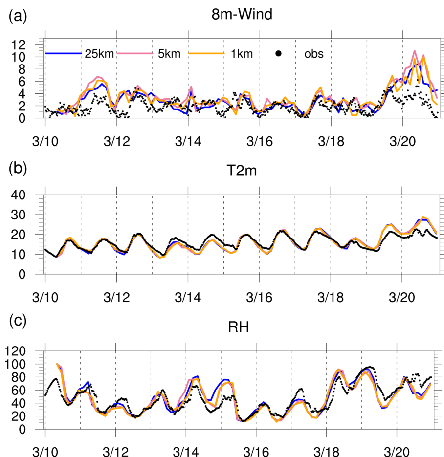
Figure 3. USTC meteorological tower observation site time series of observed (black dot) and simulated wind speed at (a) 8 m (unit: \text{m s}^{-1} ), (b) temperature at 2 m (unit: ^{\circ}\text{C} ), and (c) relative humidity (unit: %) at respective resolutions of 25 km (solid blue line), 5 km (solid pink line), and 1 km (solid orange line).
