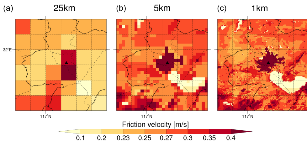
Figure 9. Spatial distribution of friction velocity in the study area for (a) 25 km, (b) 5 km, and (c) 1 km resolution simulations of the whole day. The solid black triangle indicates the location of the USTC site.
