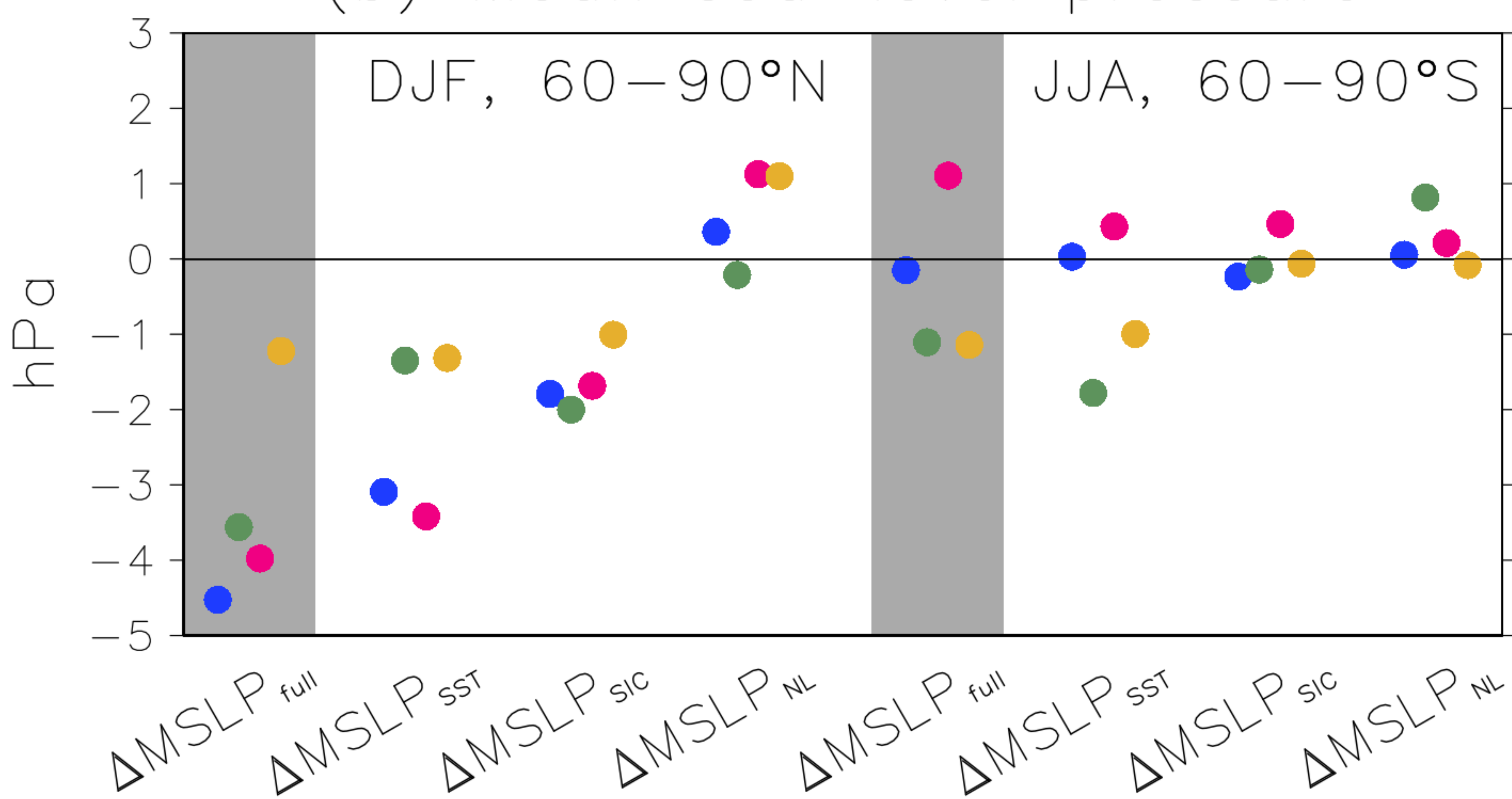
(b) Mean sea-level pressure
