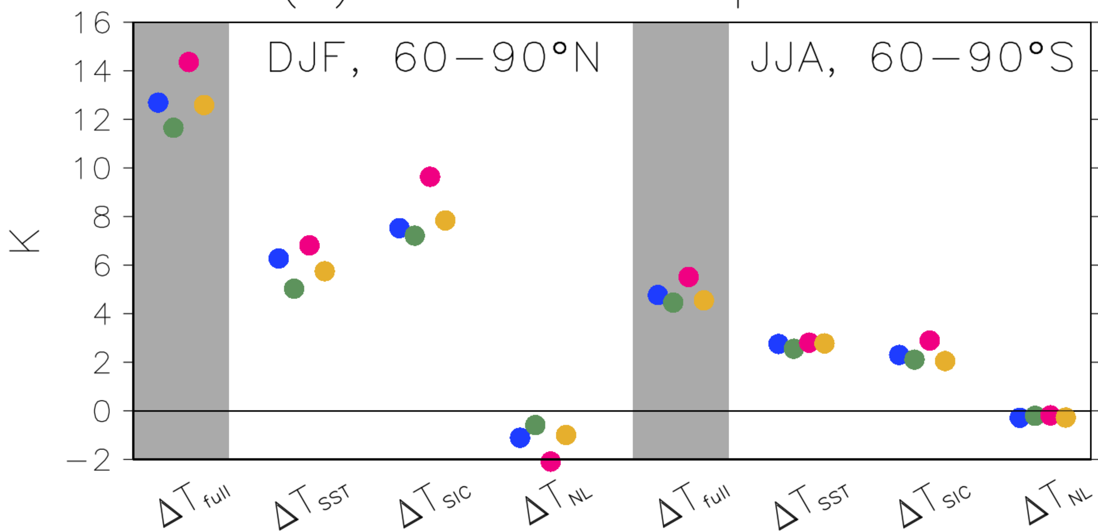
(a) 2-m air temperature
