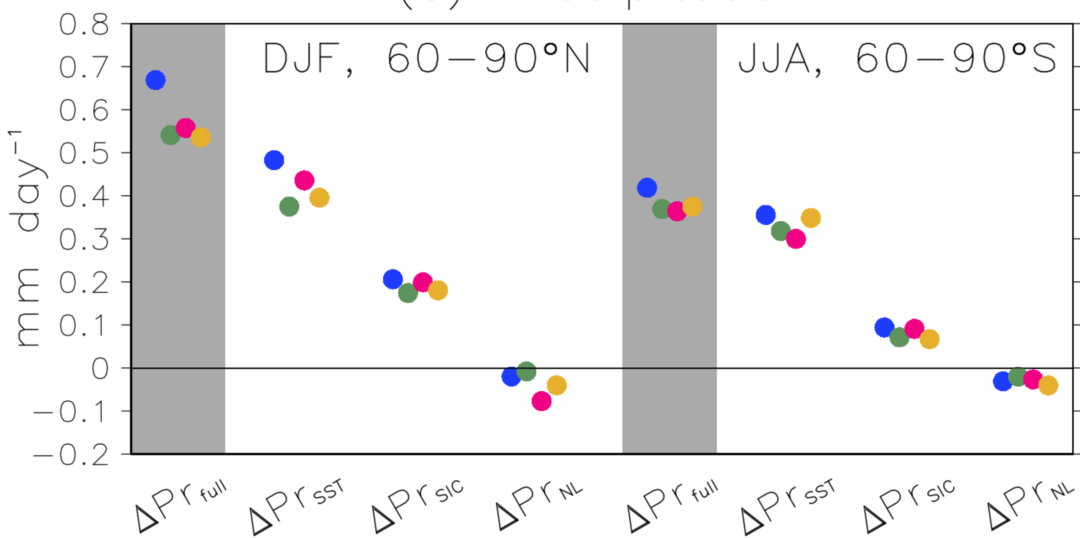
(c) Precipitation
