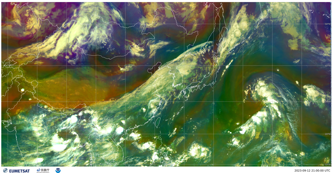
Figure S13. like Fig. S11 but for for 21 UTC on September 12, 2023.
