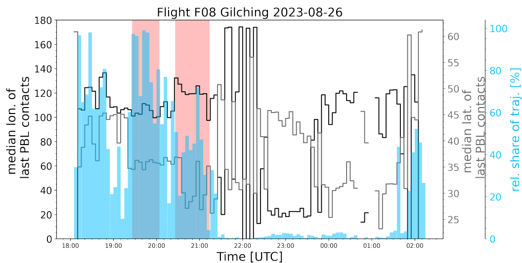
Figure S6. Flight F08 FLEXPART median latitude in grey and longitude in black of particles within the 5-min intervals. Proportion of trajectories within respective 5-minute intervals shown in blue, arriving at the PBL during the 12-day backward analysis. Major elevated time ranges are highlighted in red.
