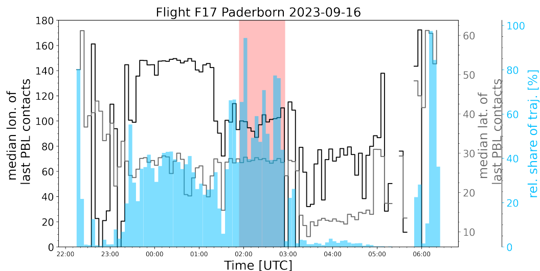
Figure S7. like Fig. S6 but for flight F17.
