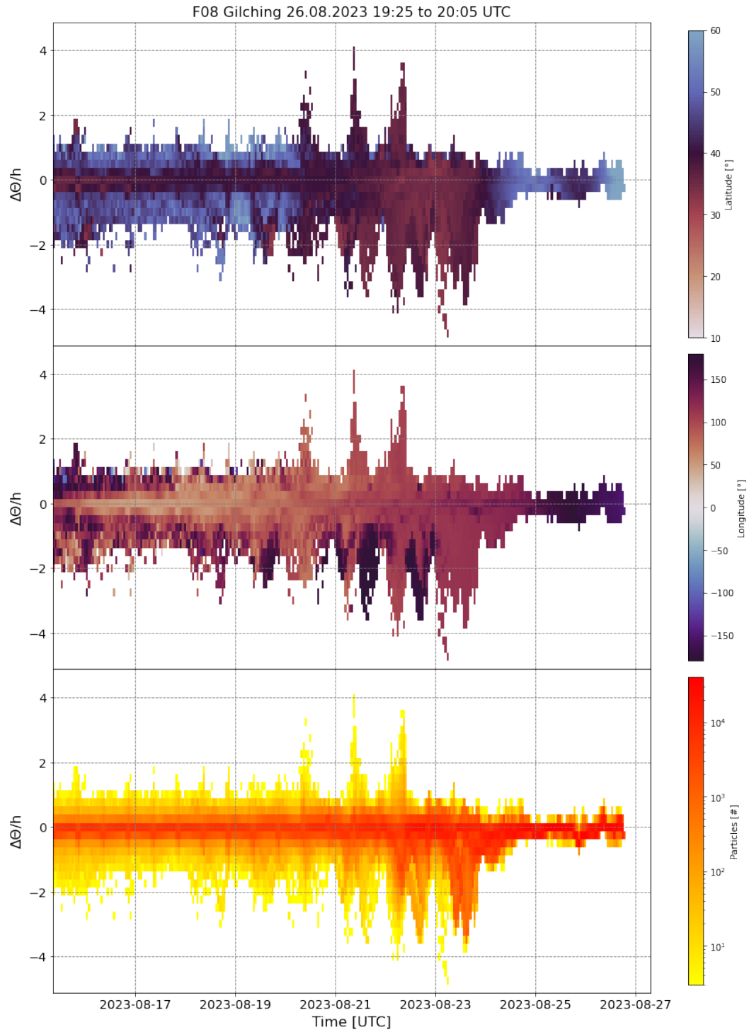
Figure S8. Hourly fluctuations in potential temperature observed along particle trajectories within the 12 days backward calculation for the first event on flight F08. Top row shows color code according to latitude, middle row according to longitude, and bottom according to particle density.
