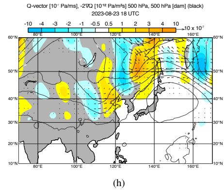
Figure S17. Q- Vector, Q-Vector vergences, and 500 hPa geopotential data for August 22 and 23, presented in 6-hourly intervals.
