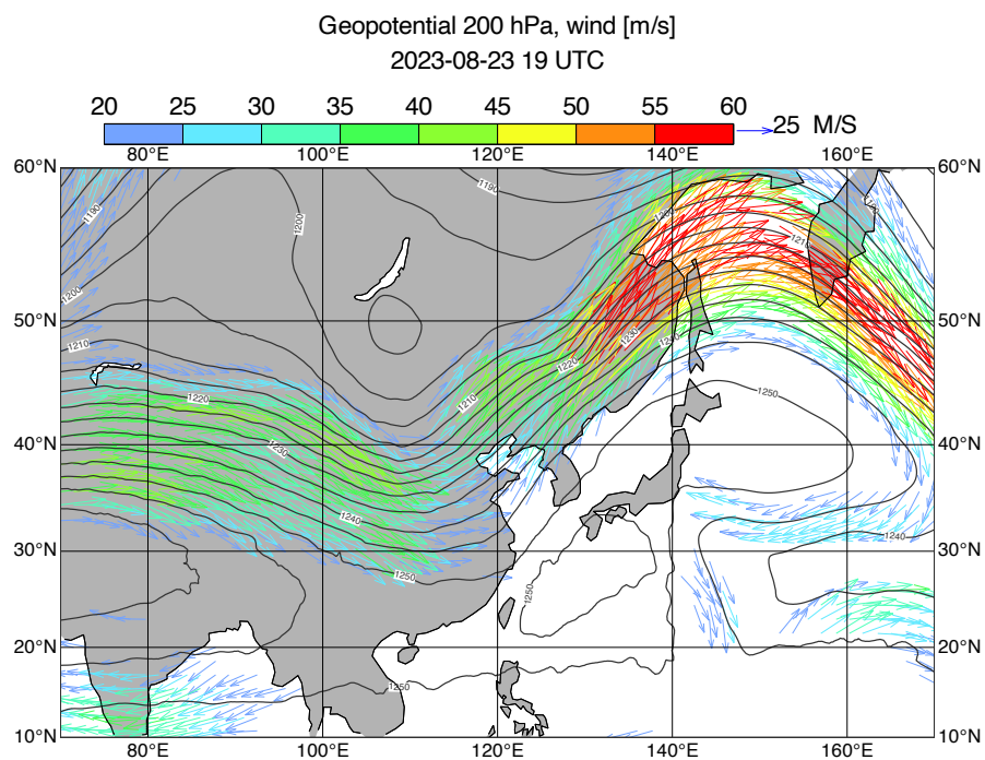
Figure S21. Upper tropospheric meteorological situation for August 23, 2023 at 19 UTC. 200 hPa geopotential heights depicted with black lines, alongside wind vectors illustrated with colored arrows. High winds speeds (orange to red arrows) show the position of the jetstreak.
