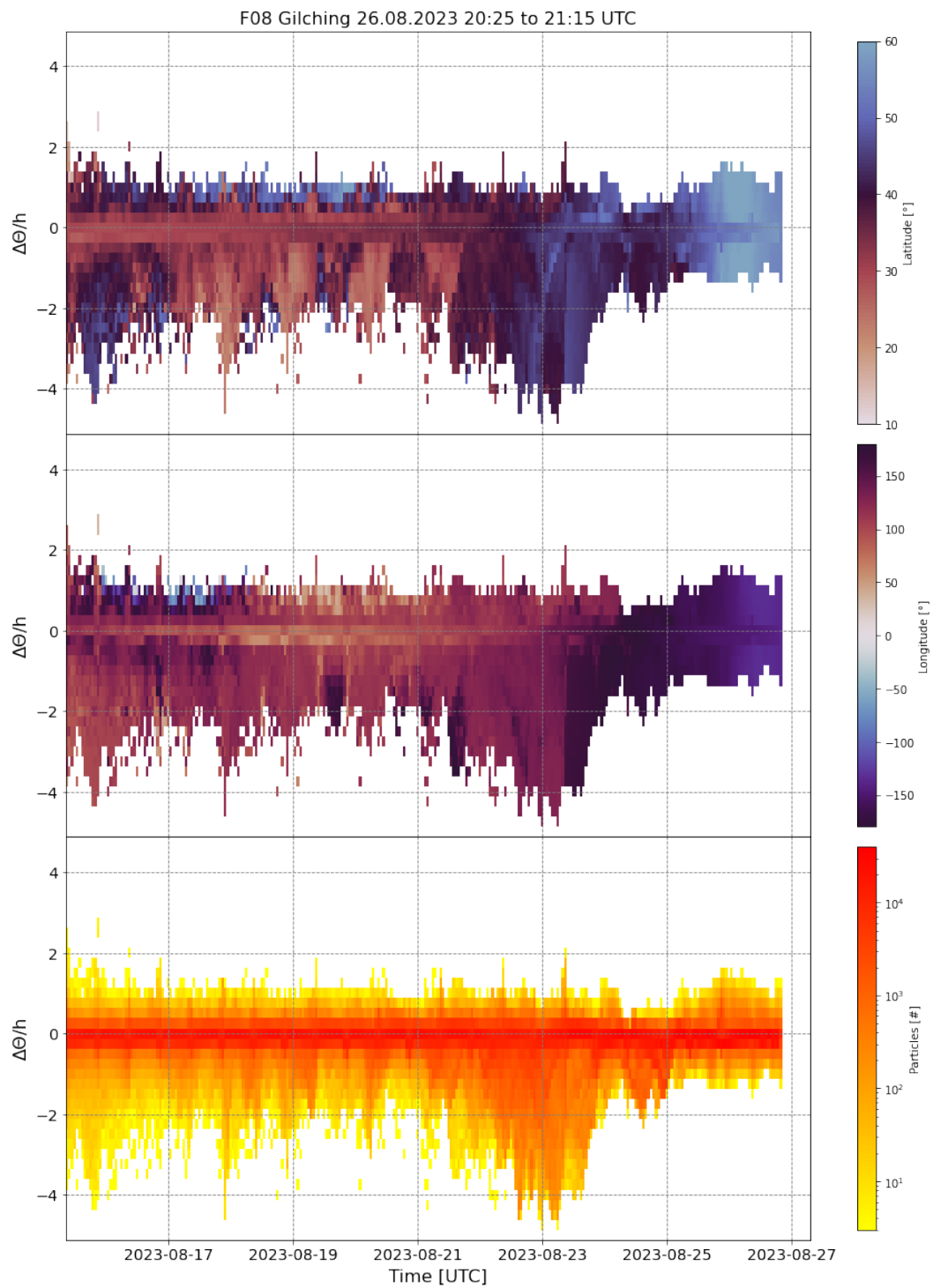
Figure S9. like Fig. S8 but for the second event on flight F08.
