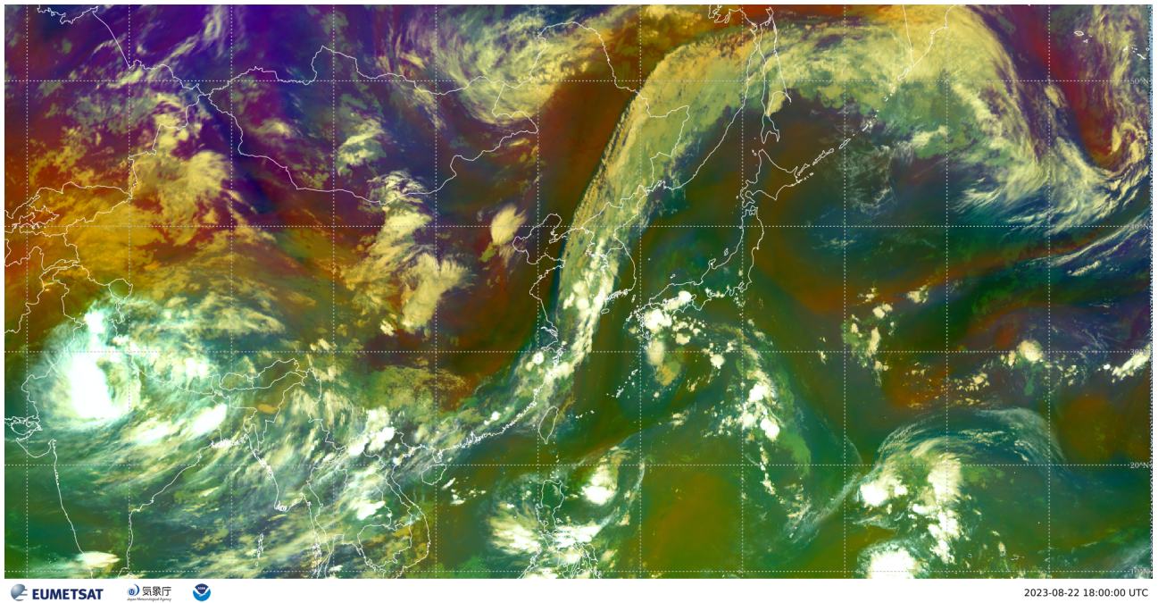
Figure S12. like Fig. S11 but for for 18 UTC on August 22, 2023.
