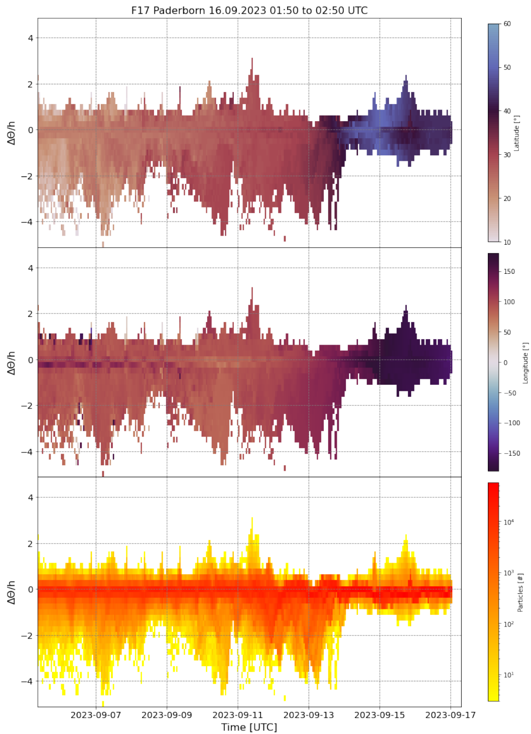
Figure S10. like Fig. S8 but for the event on flight F17.
