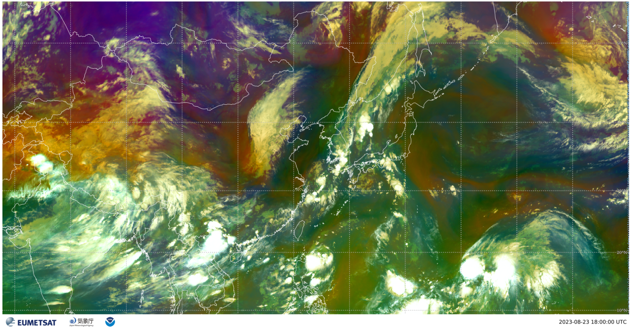
Figure S11. RGB Airmass satellite image for 18 UTC on August 23, 2023. The RGB Airmass satellite image uses the two water vapour and the ozone absorption channels. The WV6.2–WV7.3 difference (red colour beam), the IR9.7–IR10.8 difference (green colour beam), and the WV6.2 (blue colour beam). This image helps to distinguish air masses and high-reaching multi-layered clouds and to analyse dynamic processes in the atmosphere. ©EUMETSAT [2024]
