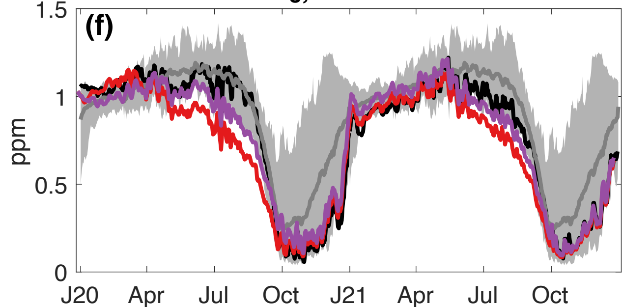
O 3 , 100 hPa
