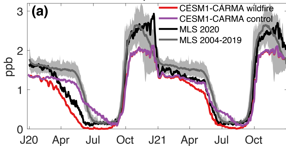
ClONO 2 , 68 hPa
