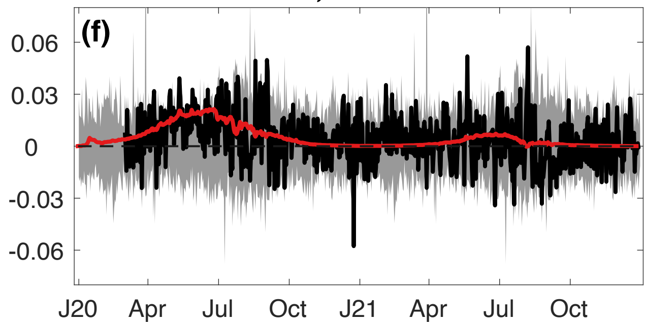
O 3 , 100 hPa
