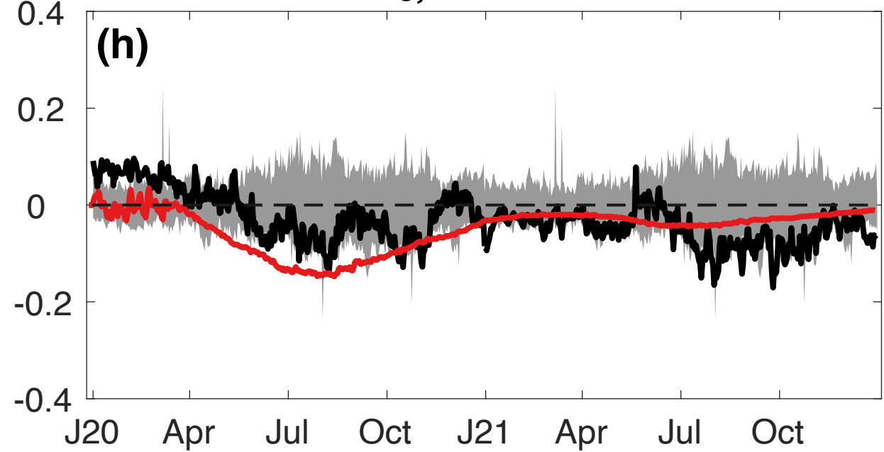
O 3 , 100 hPa
