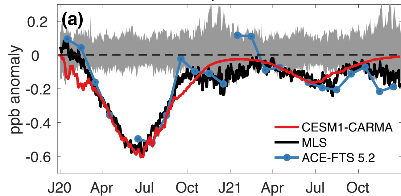
ClONO 2 , 68 hPa
