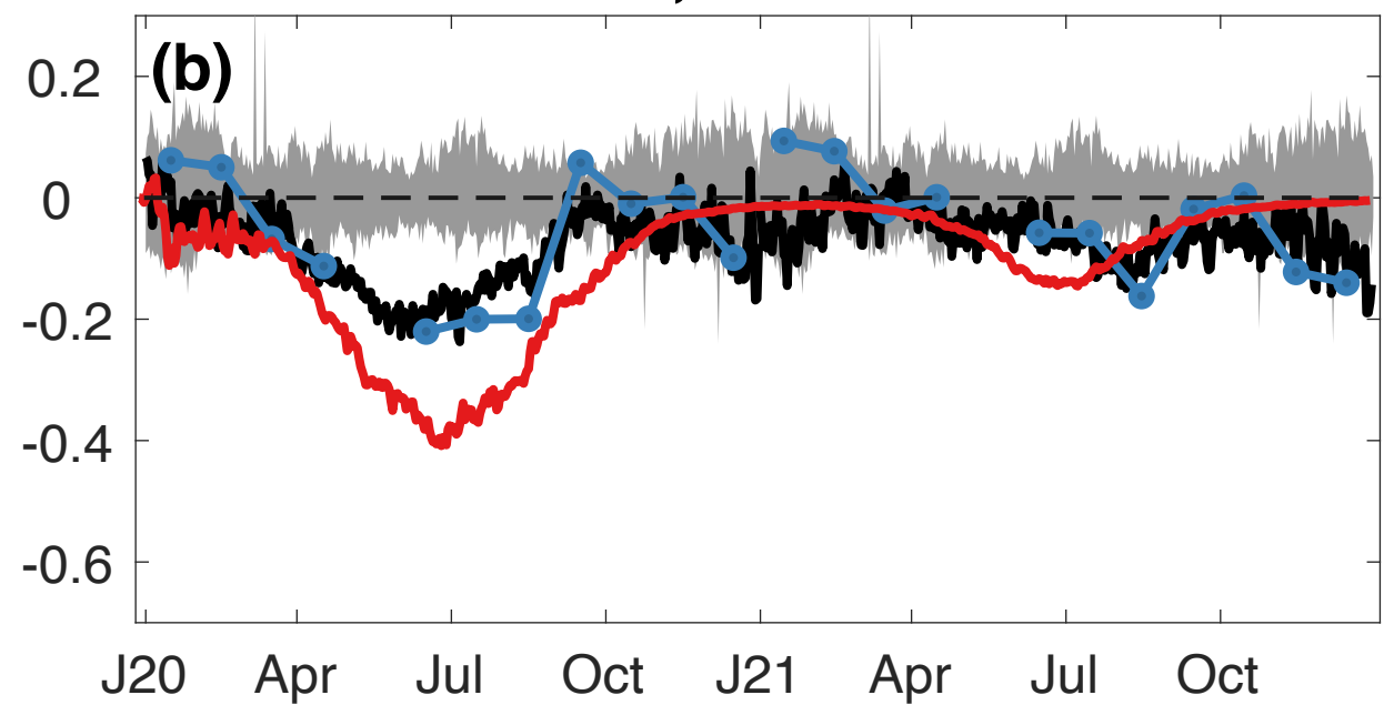
ClONO 2 , 100 hPa
