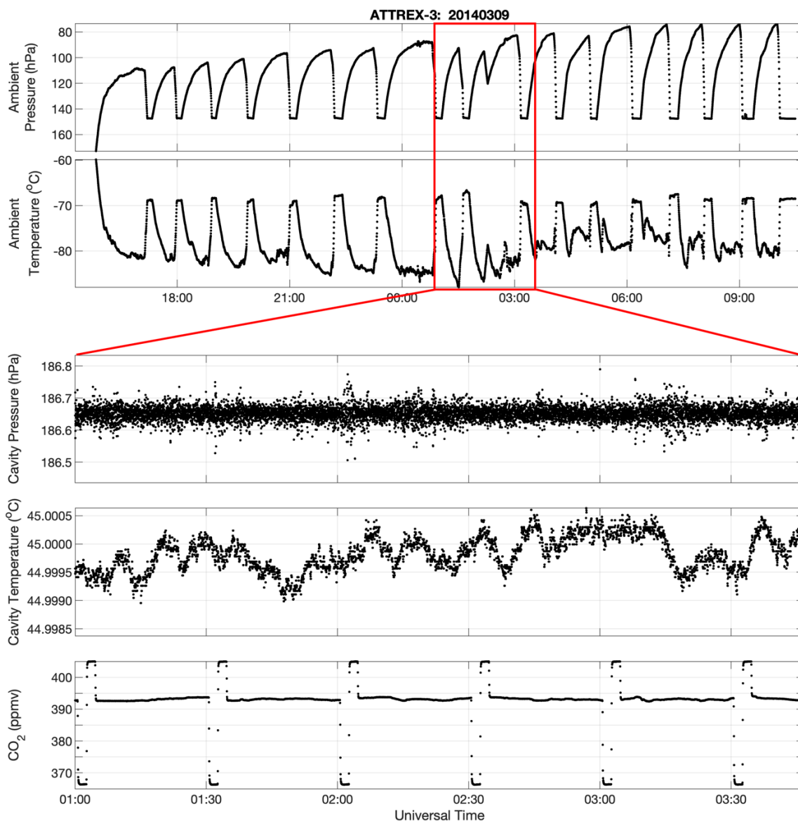
Figure S3. In-flight instrument performance during the 19.7-hour Southern Survey flight on 20140309 (ATTREX-3). Top two panels are ambient pressure and temperature. Bottom three panels are a 2.7-hr flight segment around the coldest ambient temperatures encountered during flight. Note improved Picarro cavity pressure and temperature stability as well as CO 2 precision compared to ATTREX-2 (Fig. S2).
