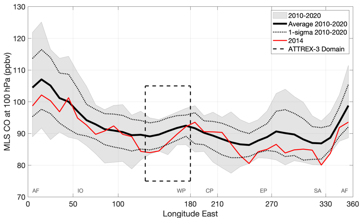
Figure S6. Ten-year record for extreme MLS CO at 100 hPa between 2010 and 2020, across the deep tropics (15° S–15° N), in February–March (Julian Days = 40–70). Extreme CO is defined as mixing ratios that are larger than two standard deviations above the average. The red line corresponds to 2014, the year of the ATTREX-3 campaign. The maximum CO at 100 hPa is consistently found over Africa. Longitudes are grouped by geographical areas: AF (Africa, 0–50° E, 345–360° E), IO (Indian Ocean, 50–100° E), WP (Western Pacific, 100–180° E), CP (Central Pacific, 180–210° E), EP (Eastern Pacific, 210–270° E), and SA (South America, 270–330° E).
