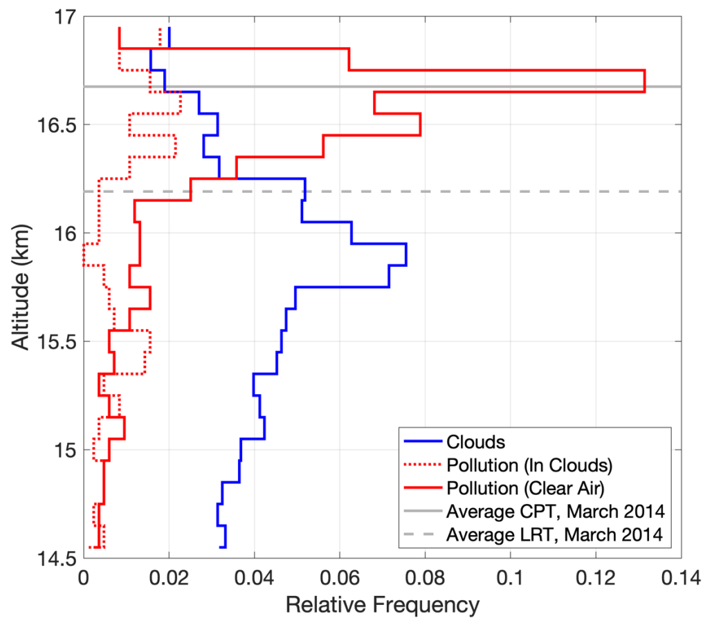
65 Figure S4. Histograms of observed clouds (blue) and pollution plumes (red) in the deep tropics (12° S–15° N) over the western Pacific in March 2014 during ATTREX-3. Clouds are defined as ice water content greater than 5 ppmv. Pollution plumes are defined as CO greater than the 80 th percentile within each latitude bin (NH: 5°–15° N, EQ: 5° S–5° N, SH: 5°–12° S). Also shown are the average altitudes of the Cold Point Tropopause (CPT) (solid gray line) and Lapse Rate Tropopause (LRT) (dashed gray line).
