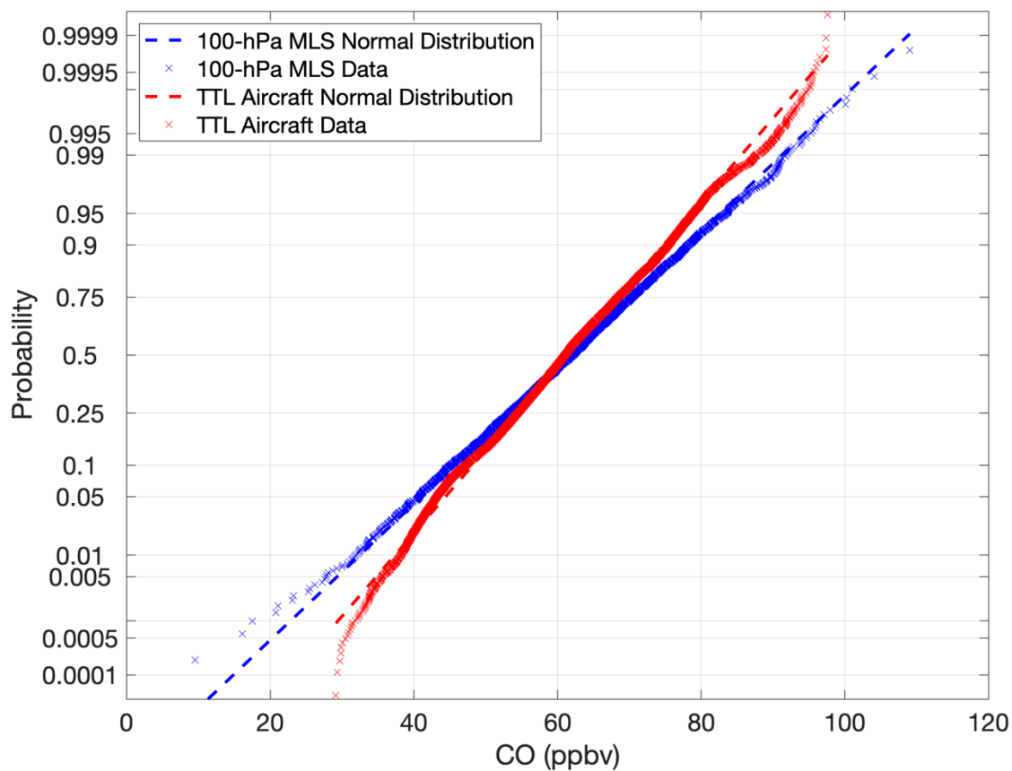
90 Figure S7. Normal probability plot comparing data and theoretical normal distributions for aircraft measurements from ATTREX-3 (red) and satellite observations from MLS (blue) over the tropical western Pacific (130–180° E) in middle February – middle March 2014. At extreme values (CO > 85 ppbv), the Kolmogorov-Smirnov test at the 95 % C.I. reveals that satellite observations are not statistically different from a normal distribution, while aircraft data depart from a normal distribution. These results indicate that the extreme high values are considered noise in the satellite data, but signal in the aircraft data.
