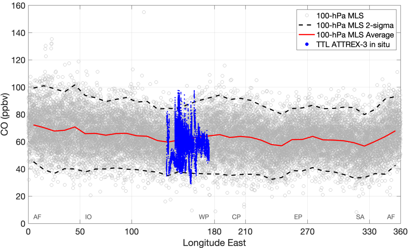
Figure S5. Aircraft in situ measurements (blue) and 100-hPa satellite observations from MLS (gray) of CO across the deep tropics (15° S–15° N) in February–March 2014. The aircraft data shown are between 80 and 140 hPa, the layer equivalent to the vertical resolution of the 100-hPa MLS CO retrieval. Longitudes are grouped by geographical areas: AF (Africa, 0–50° E, 345–360° E), IO (Indian Ocean, 50–100° E), WP (Western Pacific, 100–180° E), CP (Central Pacific, 180–210° E), EP (Eastern Pacific, 210–270° E), and SA (South America, 270–330° E).
