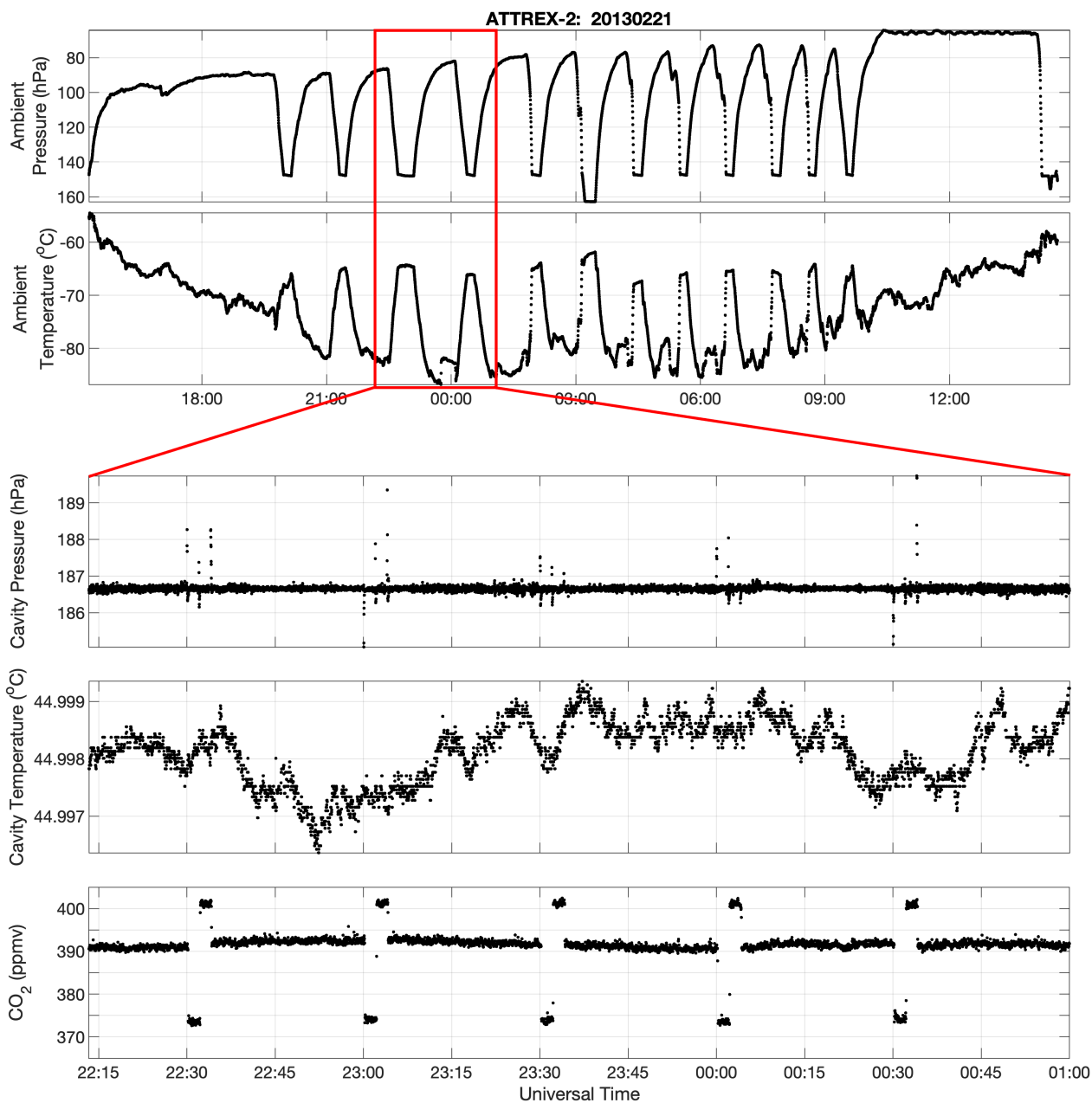
50 Figure S2. In-flight instrument performance during the 24.5-hour Southern Survey flight on 20130221 (ATTREX-2). Top two panels are ambient pressure and temperature. Bottom three panels are a 2.7-hr flight segment around the coldest ambient temperatures encountered during flight. Note the remarkable stability of the Picarro's cavity pressure and temperature and the 30-min cycling of calibration gases.
