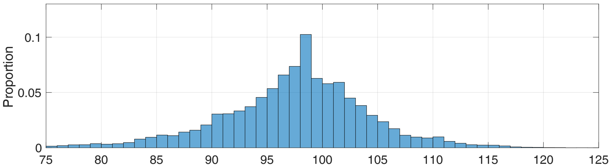
(b) RH_{ice} where 2D-S N_{Total} > 0.004 \text{ cm}^{-3} and N_{Total} \leq 0.008 \text{ cm}^{-3} (45 460 samples)
