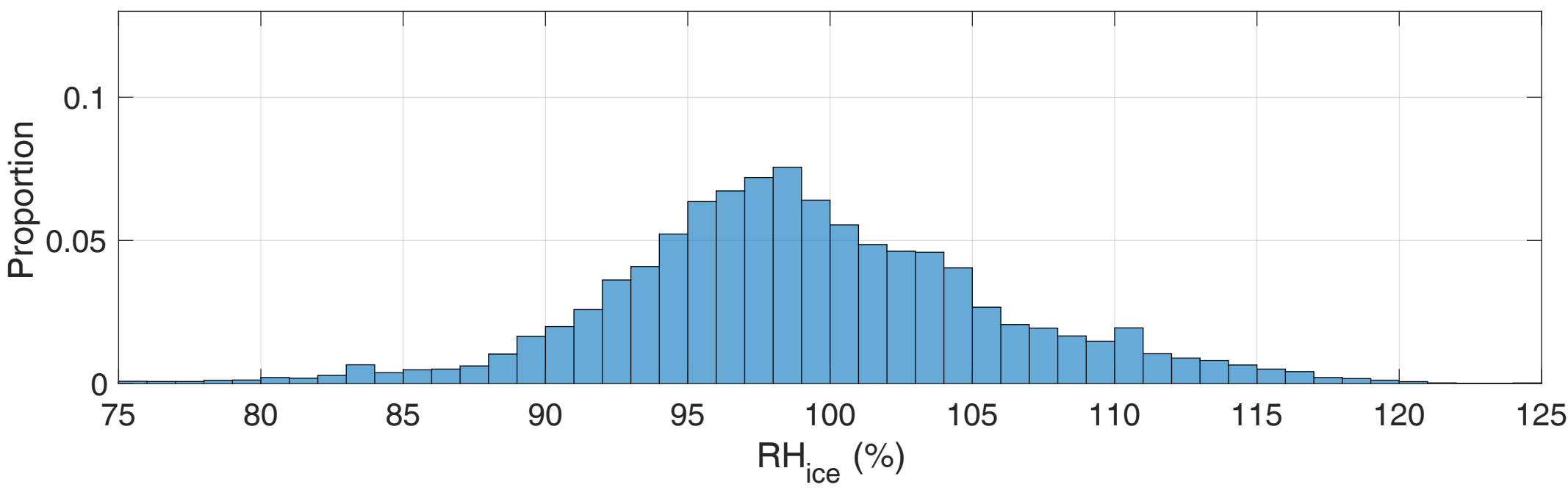
(c) RH_{ice} where 2D-S N_{Total} > 0.008 \text{ cm}^{-3} (41 138 samples)
