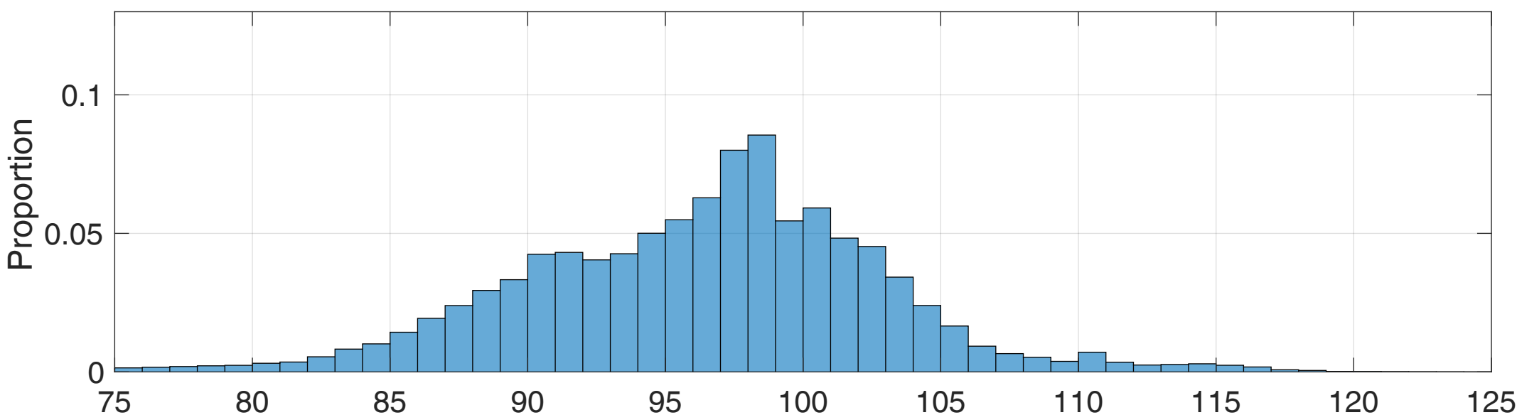
(c) RH_{ice} where 2D-S N_{Total} > 0.008 \text{ cm}^{-3} (41 138 samples)
