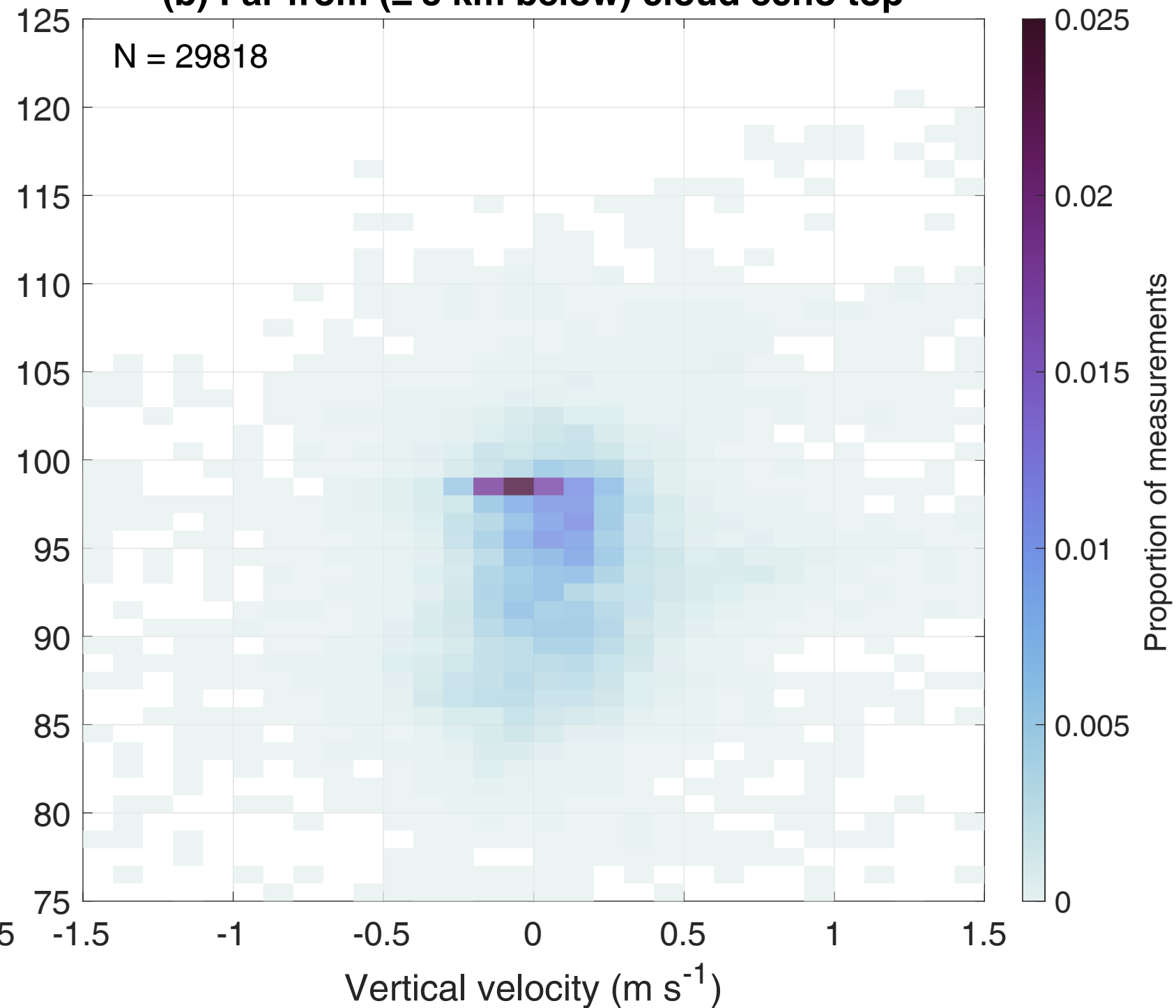
(b) Far from ( \geq 3 km below) cloud echo top
