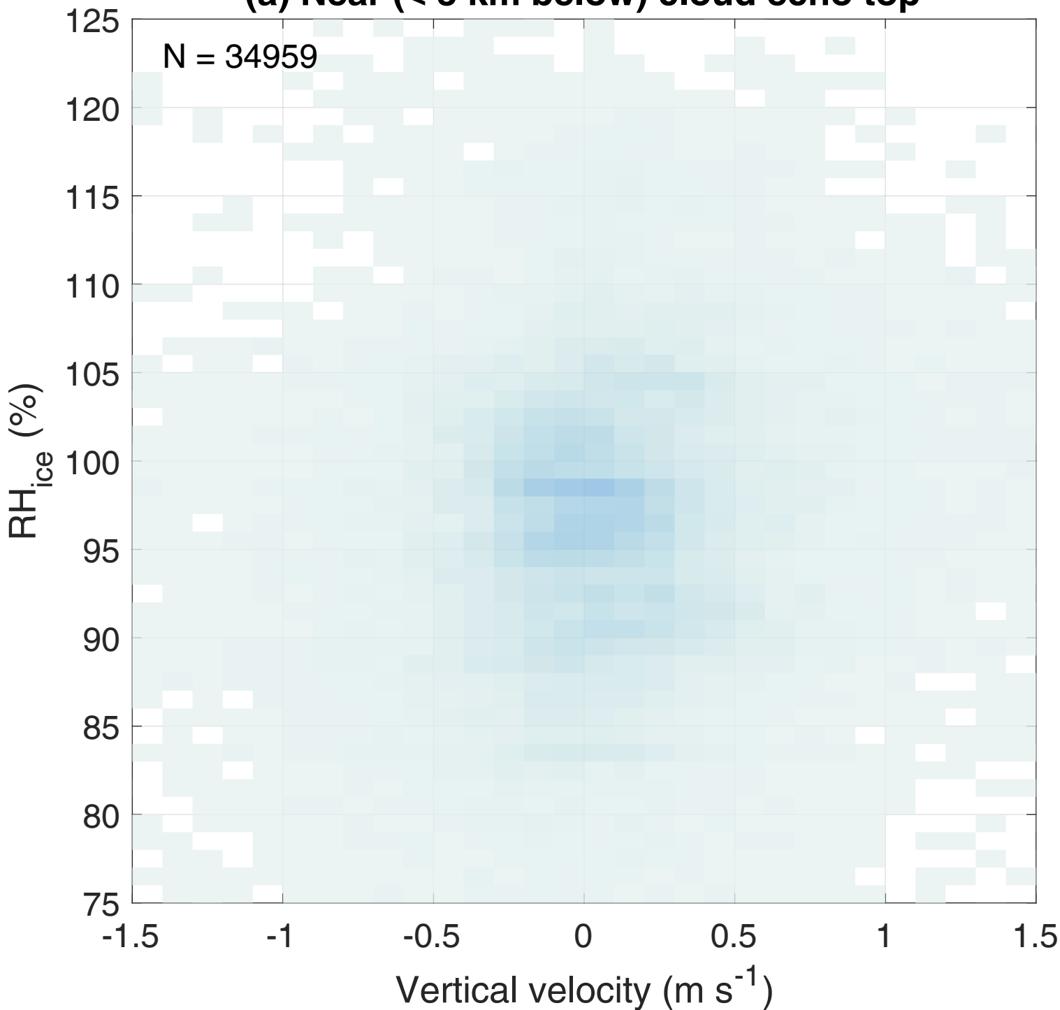
(a) Near ( < 3 km below) cloud echo top
