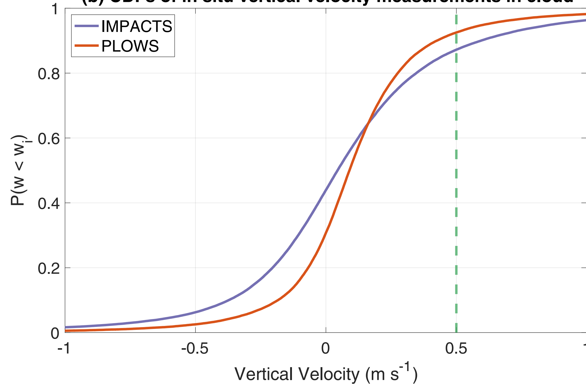
(b) CDFs of in situ vertical velocity measurements in cloud
