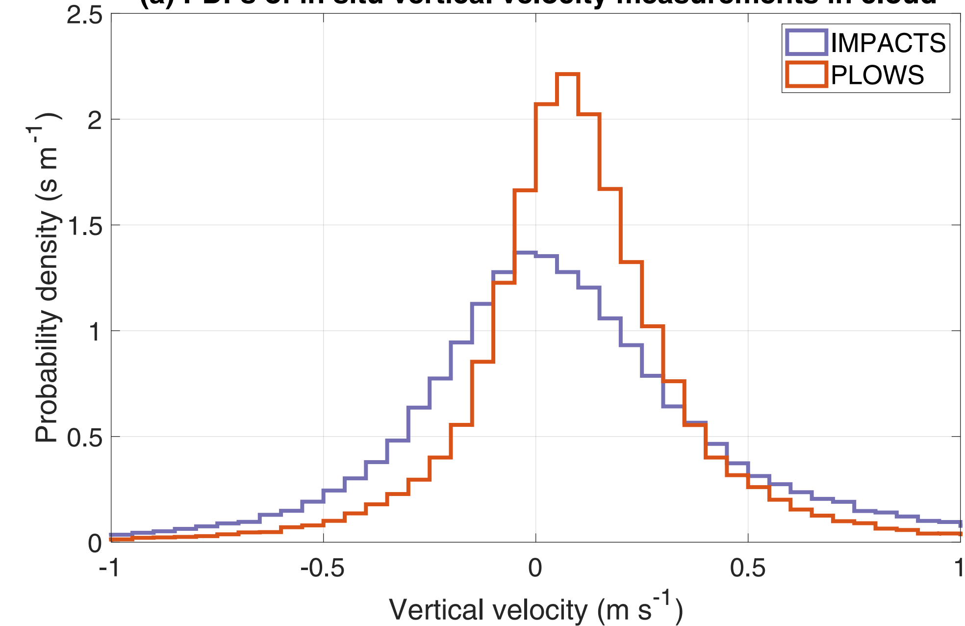
(a) PDFs of in situ vertical velocity measurements in cloud
