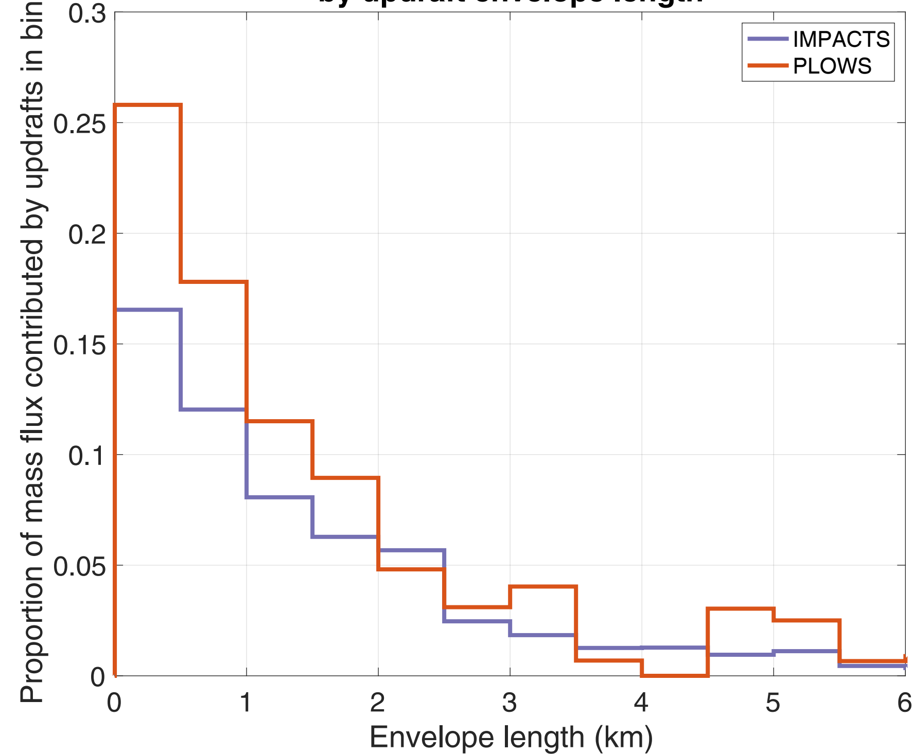
(b) Mass flux contribution by updraft envelope length
