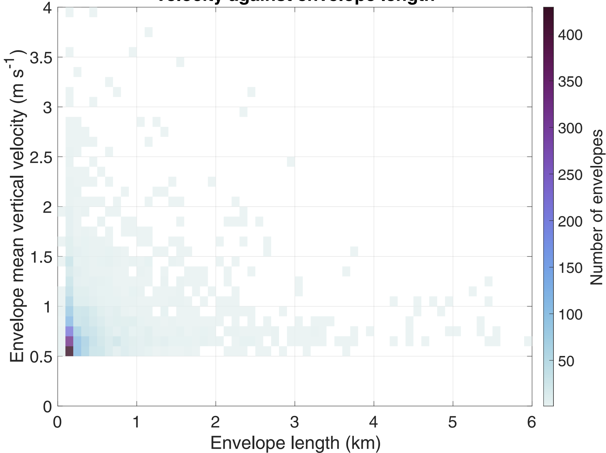
(a) IMPACTS+PLOWS envelope mean vertical velocity against envelope length
