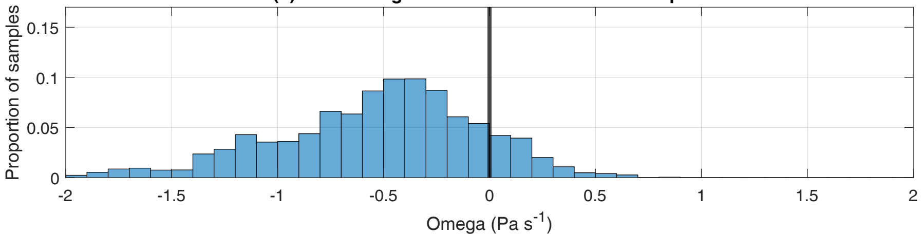
(b) ERA5 omega for all IMPACTS in-cloud samples
