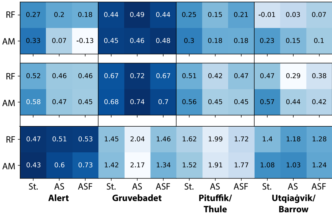
(b) Yearly cross-validation: log(MSA)
