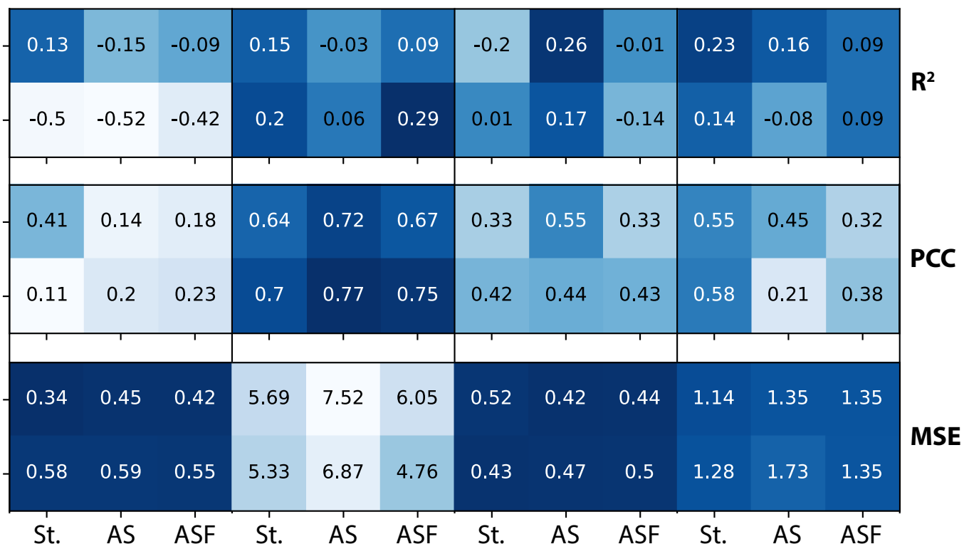
(c) Test data: MSA
