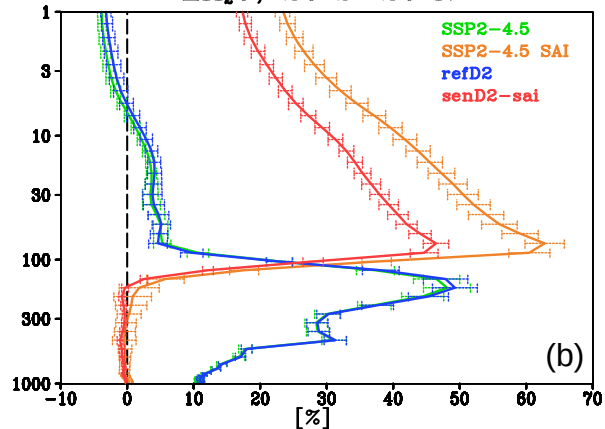
\Delta O_3 , 20°S–20°N
