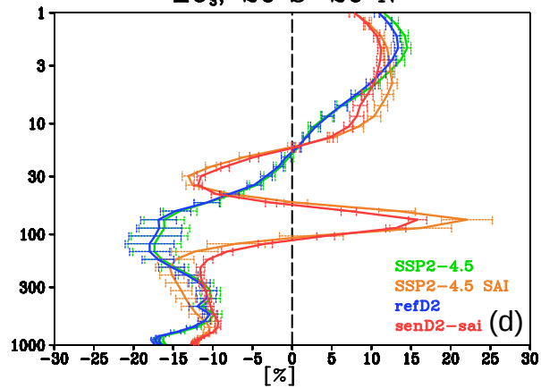
\Delta O_3 , 20°S–20°N
