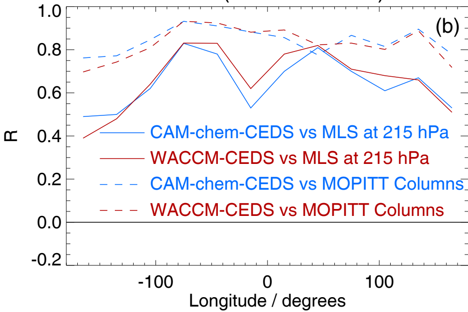
CO R values (models vs obs.): 12°S
