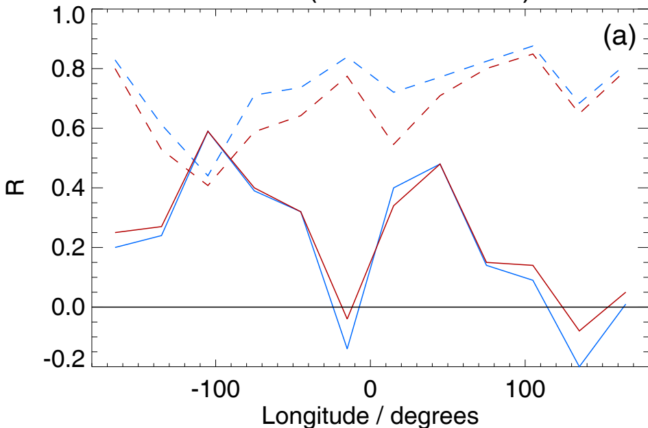
CO R values (models vs obs.): 12°N
