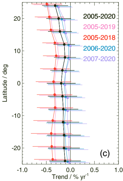
MLS CO trends at 215.4 hPa
