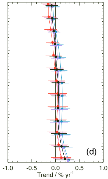
Model CO trends at 215.4 hPa
