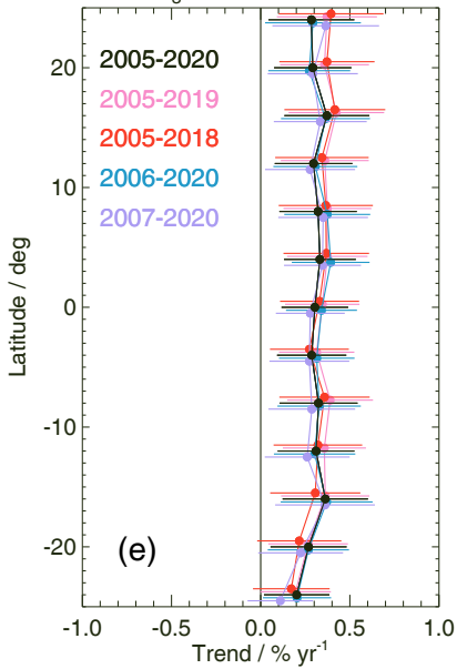
MLS O 3 trends at 215.4 hPa
