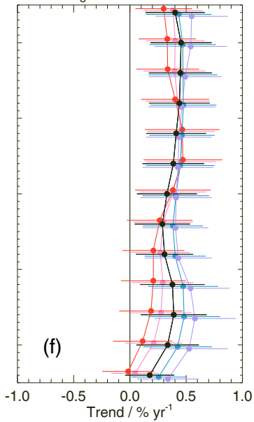
Model O 3 trends at 215.4 hPa
