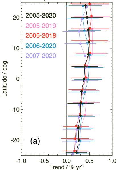
MLS O 3 trends at 177.8 hPa
