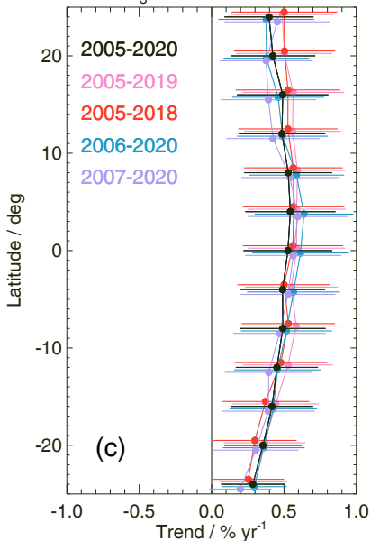
MLS O 3 trends at 215.4 hPa
