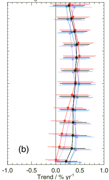
Model O 3 trends at 177.8 hPa
