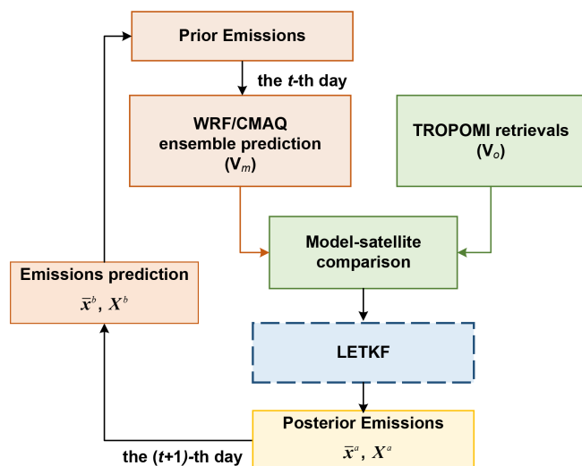
Figure 1. Flowchart of the emission inversion system.
