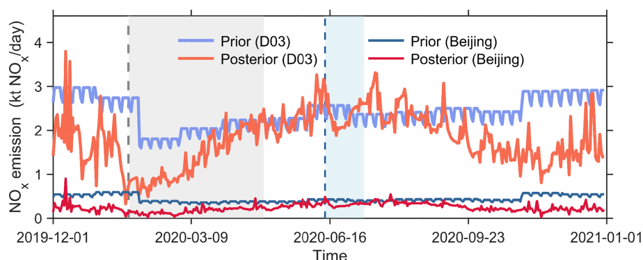
Figure 5. Time series of the bottom-up and top-down daily \text{NO}_x emissions for domain D03 and Beijing. The dashed gray line indicates the Chinese Lunar New Year, which also marks the date when Beijing began implementing COVID-19 control measures. The dashed blue line represents the start date of control measures following the sudden outbreak at the Xinfadi market in Beijing. The gray shaded area represents the period affected by COVID-19 measures in 2020, and the light blue shaded area highlights the time frame impacted by the Xinfadi market outbreak.
