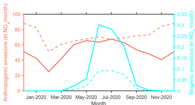
Figure 6. Monthly \text{NO}_x emissions from the grids dominated by anthropogenic (red) and biogenic (cyan) sources. The solid and dashed curves represent the posterior and the prior \text{NO}_x emissions, respectively.
