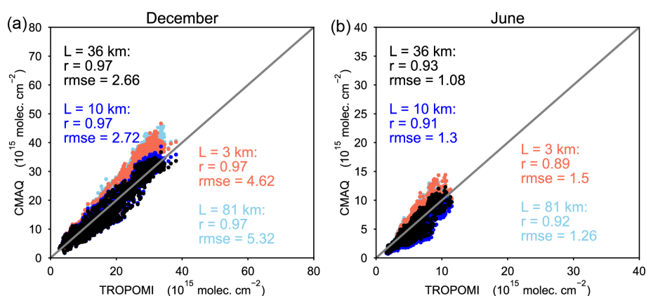
Figure 9. Scatterplots of the TROPOMI NO 2 TVCDs and the CMAQ simulated NO 2 TVCDs from the inversion experiments with a localization parameter of 3, 10, 36, and 81 km, respectively. (a) December 2019. (b) June 2020.
