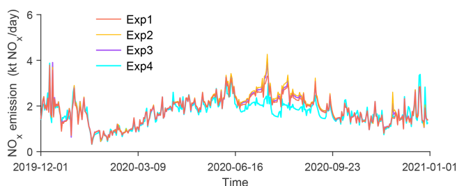
Figure 7. The daily posterior emission time series from the sensitivity experiments Exp1–Exp4 in the domain D03.
