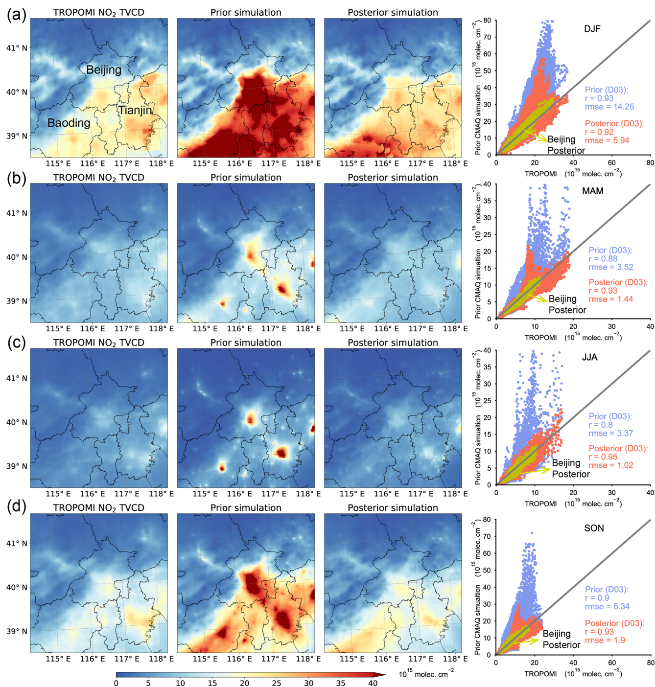
Figure 2. Comparison of the spatial distributions of TROPOMI \text{NO}_2 TVCD retrievals (the left column) with CMAQ-modeled \text{NO}_2 TVCDs driven by the prior (the second column) and posterior (the third column) emissions. The CMAQ-modeled \text{NO}_2 TVCDs are calculated using satellite averaging kernels. The last column is the scatterplot of the TROPOMI retrievals with the CMAQ-modeled \text{NO}_2 TVCDs simulated using the prior (blue) and posterior (red) emissions. From top to bottom, the rows represent winter (DJF), spring (MAM), summer (JJA), and autumn (SON).
