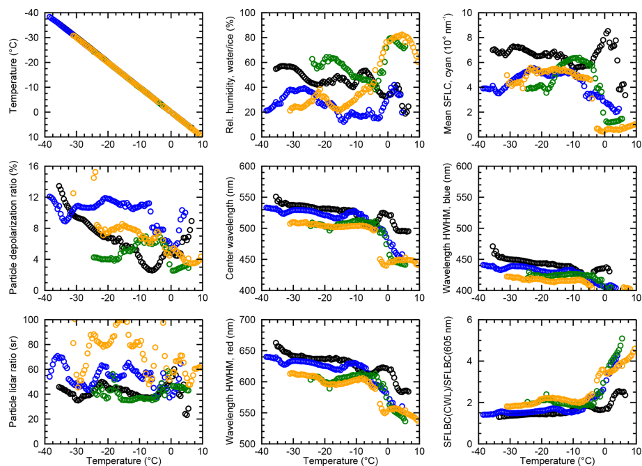
Figure A11. Similar to Fig. A10, but for ambient temperature as the independent variable. Data points have a bin width of 0.5 K, and mean values are shown.
