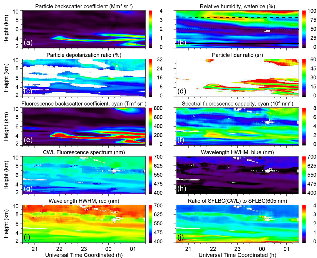
Figure A6. Similar to Fig. A1, but for the RAMSES measurement in the night of 1–2 June 2023 between 20:30 and 01:30 UTC. Black lines in panel (b) indicate 0, -20, and -40 °C isotherms.
