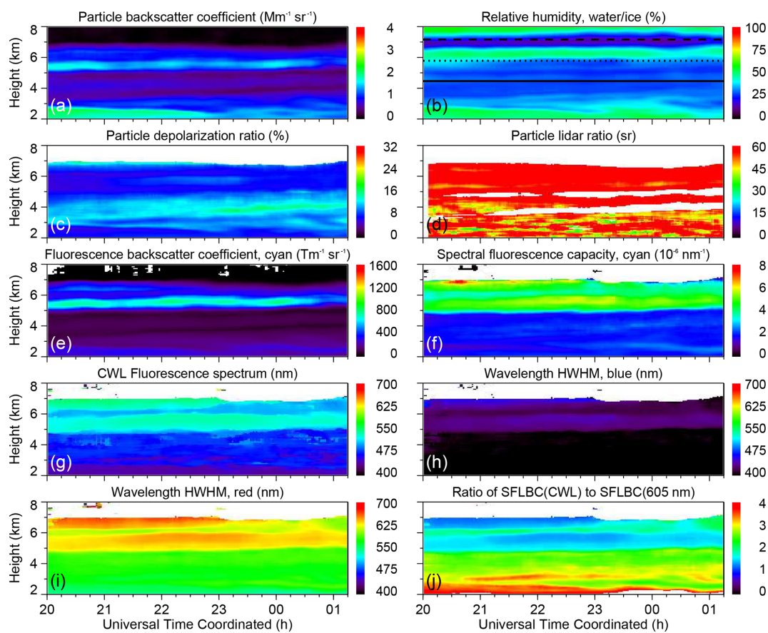
Figure A5. Similar to Fig. A1, but for the RAMSES measurement in the night of 20–21 July 2022 between 20:00 and 01:15 UTC. Black lines in panel (b) indicate 0, -10, and -20 °C isotherms.
