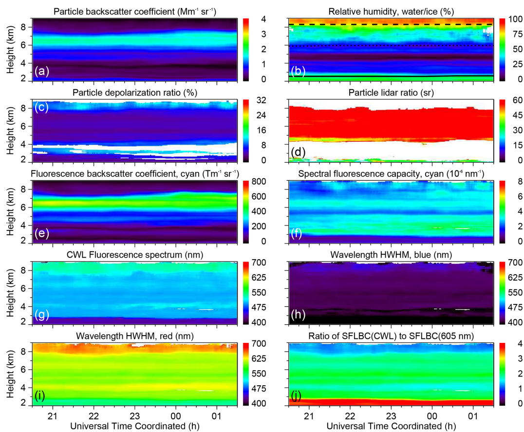
Figure A7. Similar to Fig. A1, but for the RAMSES measurement in the night of 4–5 June 2023 between 20:30 and 01:30 UTC. Black lines in panel (b) indicate 0, -20, and -40 °C isotherms.
