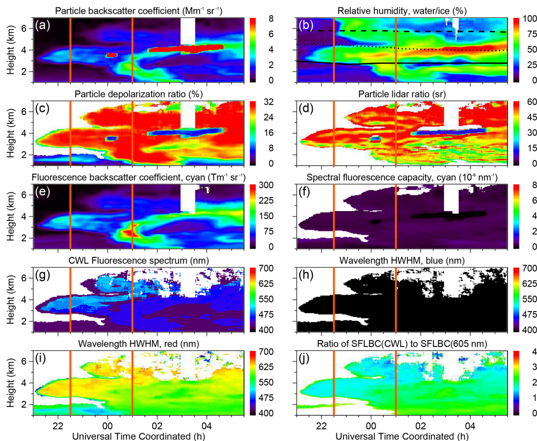
Figure 7. Similar to Fig. 4, but for the RAMSES measurement in the night of 22–23 February 2021 between 21:00 and 05:30 UTC. Black lines in panel (b) indicate 0, –10, and –20 °C isotherms. The measurements at 22:30 and 01:00 UTC (times marked by vertical orange lines) are analyzed in Figs. 8 and 9.
