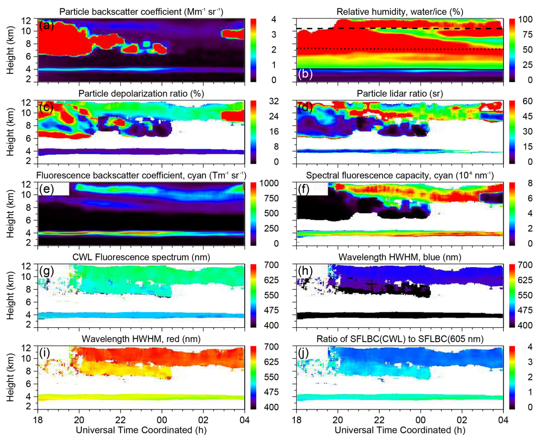
Figure A3. Similar to Fig. A1, but for the RAMSES measurement in the night of 19–20 September 2020 between 18:00 and 04:00 UTC. Black lines in panel (b) indicate 0, -25, and -50 °C isotherms.
