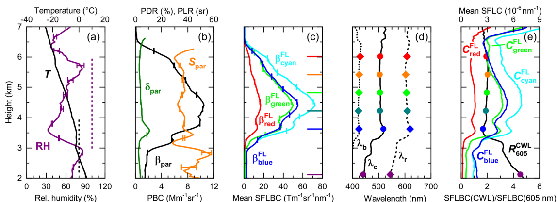
Figure 5. Measurement of the BBA layer at 22:30 UTC on 4 July 2023. Profiles of (a) relative humidity with respect to water or ice (RH; saturation level indicated by a vertical dashed violet line) and temperature ( T ; freezing temperature indicated by a vertical dashed black line), (b) particle backscatter coefficient (PBC, \beta_{\text{par}} ), particle depolarization ratio (PDR, \delta_{\text{par}} ) and particle lidar ratio (PLR, S_{\text{par}} ), (c) mean spectral fluorescence backscatter coefficients (SFLBC, \beta^{\text{FL}} ) for the spectral bands ranging from 430–450 nm (blue), 455–535 nm (cyan), 545–625 nm (green), and 630–710 nm (red), (d) wavelength of the maximum of the fluorescence spectrum (CWL, \lambda_c ), wavelength of the spectrum half-width on the blue shoulder ( \lambda_b ) and wavelength of the spectrum half-width on the red shoulder ( \lambda_r ), and (e) ratio of CWL to 605 nm spectral fluorescence backscatter coefficients ( R_{605}^{\text{CWL}} ) and mean spectral fluorescence capacities (SFLC, C^{\text{FL}} ) for the blue, cyan, green, and red spectral bands (colored curves). Colored symbols and horizontal lines indicate altitudes for which the fluorescence spectra are presented in Fig. 6. Data integration time is 1200 s. The resolution of the raw data is 60 m, and signal profiles are smoothed with a sliding average length increasing with height. Bars in panels (a)–(c) indicate statistical errors of the lidar measurement (omitted in panels d and e for the sake of conciseness). Temperature profiles were obtained by interpolating data from radiosondes launched every 6 h on-site.
