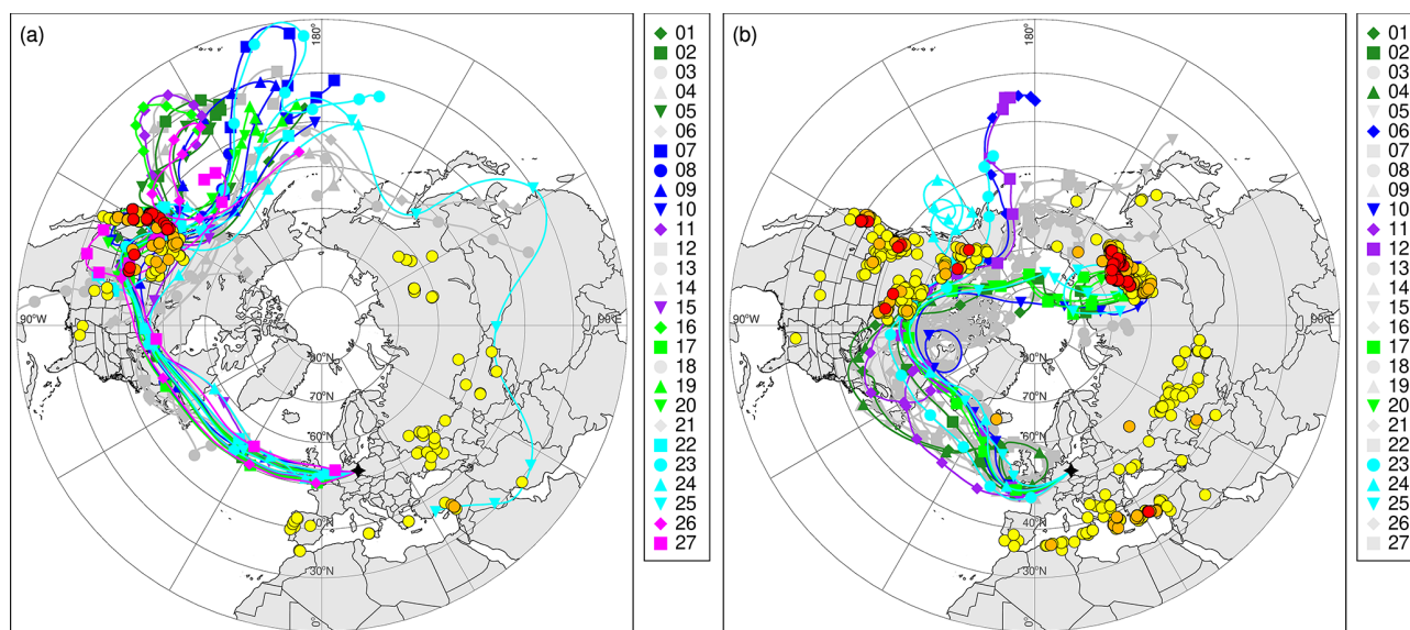
Figure 2. Two examples of the HYSPLIT back-trajectory ensemble for the starting points (a) 12 September 2020 at 01:00 UTC and 5.0 km altitude and (b) 9 August 2021 at 23:00 UTC and 5.4 km altitude. Trajectories close to fires are indicated by colored lines and symbols, and all other trajectories of the ensemble are shown in gray. Fires are represented by filled circles and color-coded according to the accumulated fire radiative power (FRP) of a fire region; yellow, orange, and red circles indicate FRP values between 500 and 5000, 5000 and 25000, and > 25000 \text{ Wm}^{-2} , respectively.
