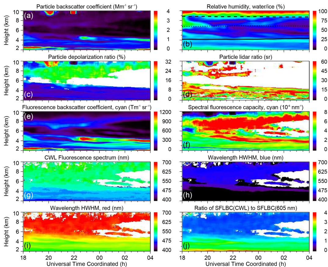
Figure A2. Similar to Fig. A1, but for the RAMSES measurement in the night of 13–14 September 2020 between 18:00 and 04:00 UTC. Black lines in panel (b) indicate 0, -15, and -30 °C isotherms.
