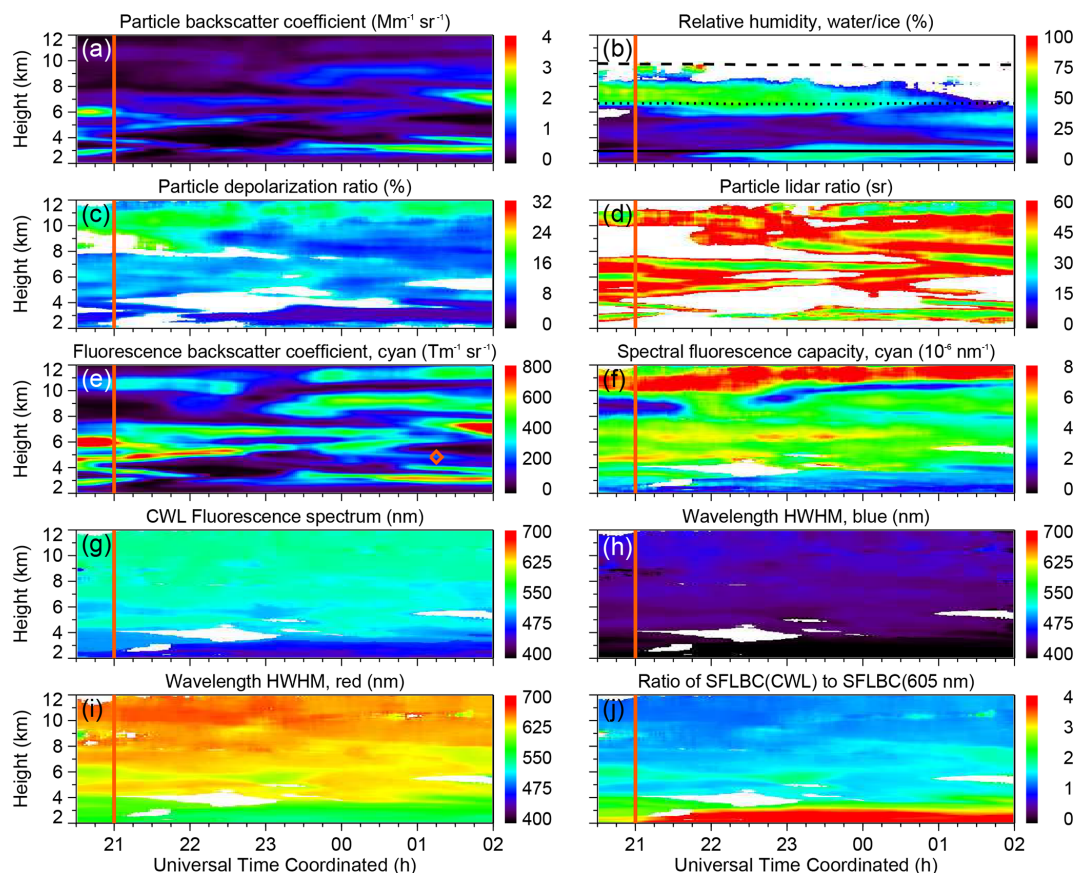
Figure 10. Similar to Fig. 4, but for the RAMSES measurement in the night of 26–27 May 2023 between 20:30 and 02:00 UTC. Black lines in panel (b) indicate 0, −25, and −50 °C isotherms. The measurement at 21:00 UTC (time marked by a vertical orange line) is analyzed in Figs. 11 and 12, and the spectrum measured at 4.8 km around 01:15 UTC (orange symbol, panel e) is shown in Fig. 1.
