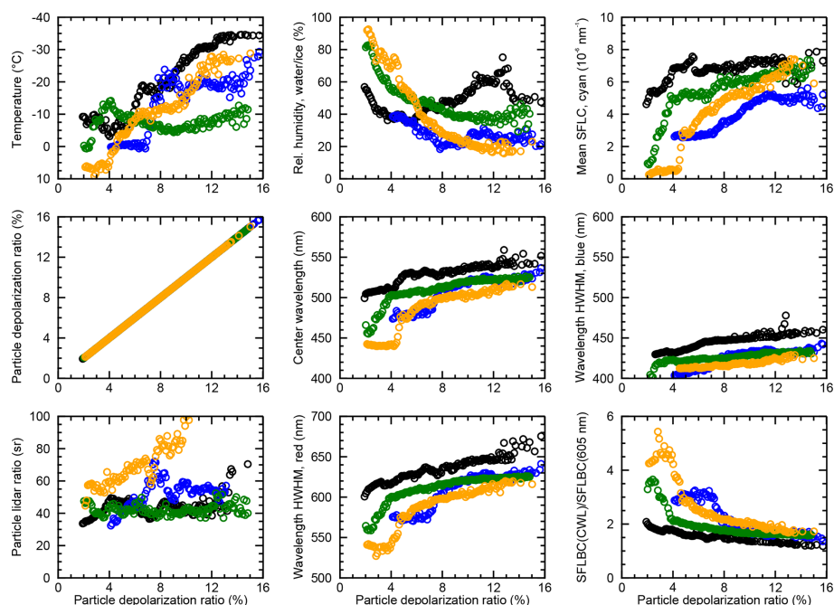
Figure A10. Dependence of selected atmospheric variables and elastic and inelastic aerosol properties on the particle depolarization ratio. Data points have a bin width of 0.1 % (absolute), and mean values are shown. Measurement nights and data ranges are the same as in Fig. 15. Results for 11–12 September 2020, 26–27 May 2023, 4–5 July 2023, and 9–10 July 2023 are illustrated with black, blue, green, and orange symbols, respectively.
