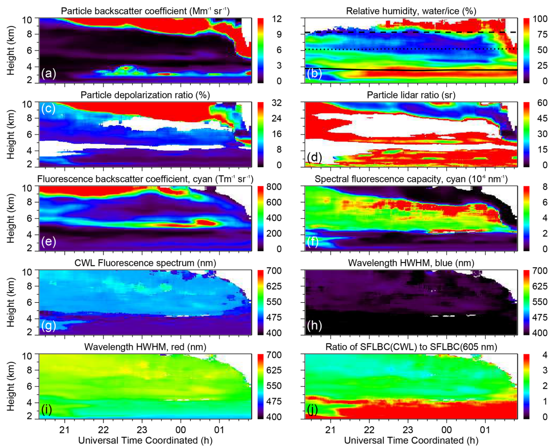
Figure A8. Similar to Fig. A1, but for the RAMSES measurement in the night of 9–10 July 2023 between 20:20 and 01:50 UTC. Black lines in panel (b) indicate 0, -15 , and -30 °C isotherms.
