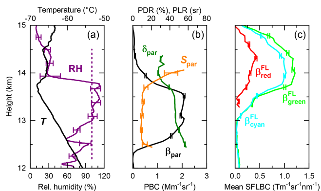
Figure 18. Measurement at 23:45 UTC on 13 September 2020. Profiles of (a) relative humidity with respect to ice (RH; saturation level indicated by a vertical dashed violet line) and temperature ( T ), (b) particle backscatter coefficient (PBC, \beta_{\text{par}} ), particle depolarization ratio (PDR, \delta_{\text{par}} ) and particle lidar ratio (PLR, S_{\text{par}} ; not corrected for multiple scattering), and (c) mean spectral fluorescence backscatter coefficients (SFLBC, \beta^{\text{FL}} ) for the cyan, green, and red spectral bands. T and RH profiles were measured with the routine RS41 radiosonde launched at 22:45 UTC on-site. Bars indicate statistical measurement errors (RAMSES) or total measurement uncertainty (RS41).
