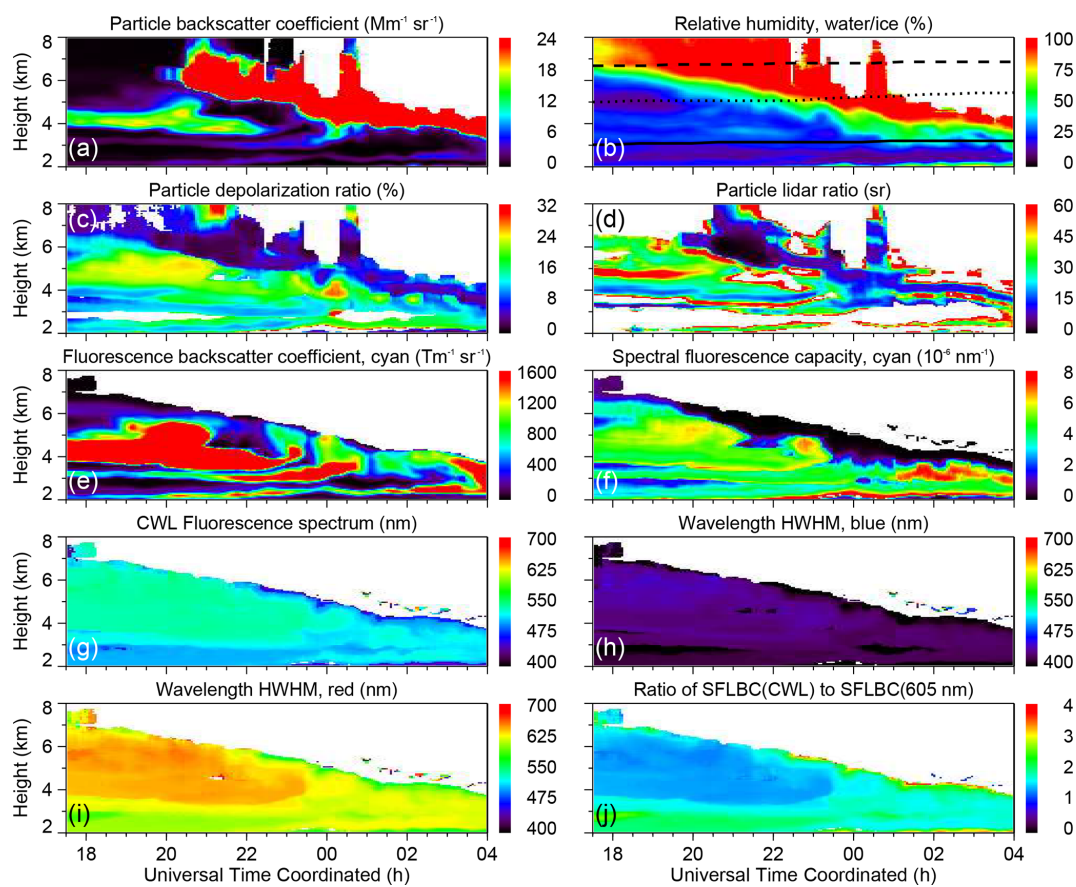
Figure A9. Similar to Fig. A1, but for the RAMSES measurement in the night of 30 September–1 October 2023 between 17:30 and 04:00 UTC. Black lines in panel (b) indicate 0, -10, and -20 °C isotherms.
