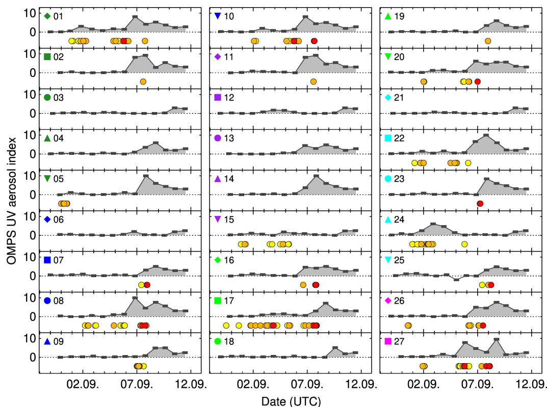
Figure 3. OMPS aerosol index values along the path of the 27 ensemble trajectories (horizontal gray bars) for the starting point 12 September 2020 at 01:00 UTC and 5 km (Fig. 2a). Fires close to trajectories are indicated by filled circles, and the colors match those in Fig. 2.
