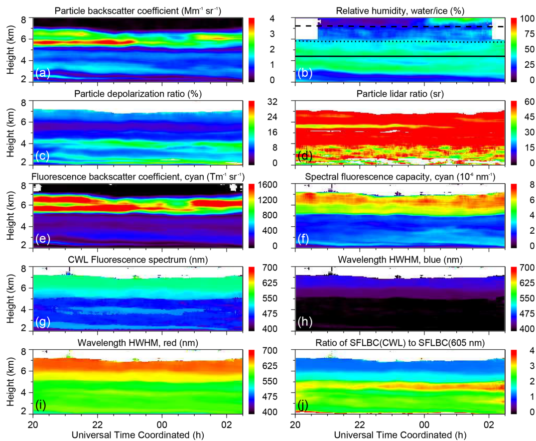
Figure A4. Similar to Fig. A1, but for the RAMSES measurement in the night of 19–20 July 2022 between 20:00 and 02:30 UTC. Black lines in panel (b) indicate 0, −10, and −20 °C isotherms.
