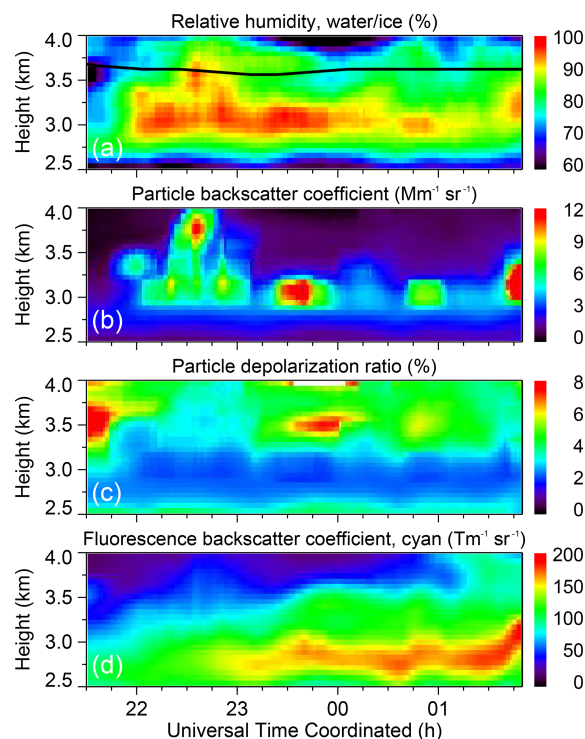
Figure 21. Temporal evolution of (a) relative humidity (with respect to water and ice above and below 0 °C, respectively; 0 °C isotherm indicated by a black line), (b) particle backscatter coefficient, (c) particle depolarization ratio, and (d) fluorescence backscatter coefficient (cyan false color: spectrum integrated from 455 to 535 nm) as measured with RAMSES in the night of 9–10 July 2023 between 21:30 and 01:50 UTC. The data shown are a section of the night-long measurement (Fig. A8).
