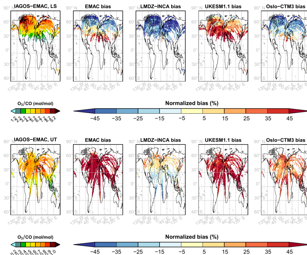
Figure A1. Same as Fig. 1 but for the O_3/CO ratio over the period from 2002 to 2017.
