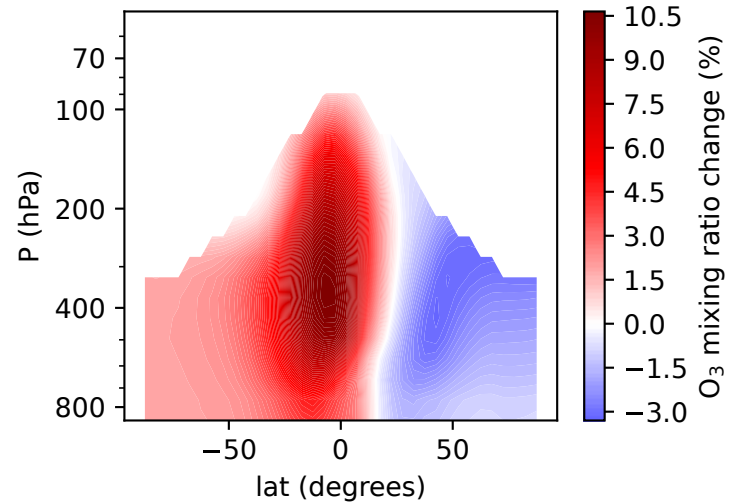
(f) 100 \times (\text{LNOfs}_G - \text{CTR}_G) / \text{CTR}_G
