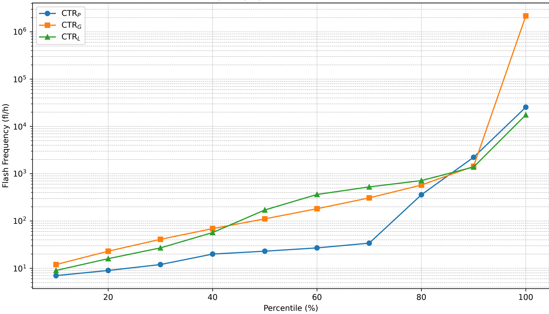
Flash Frequency by Percentile for CTR Simulations
