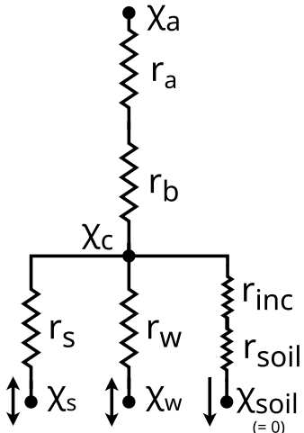
DEPAC scheme
