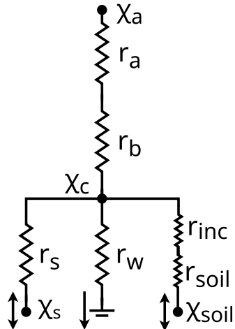
Zhang scheme
