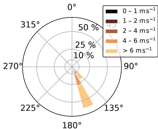
(a) ERA5 at Galapagos
