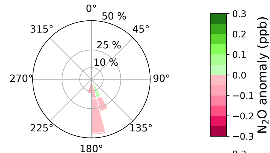
(c) N 2 O Observations
