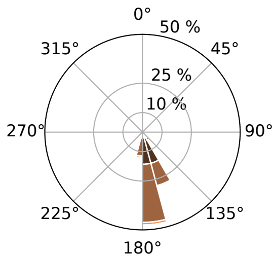
(b) GSC Meteorology
