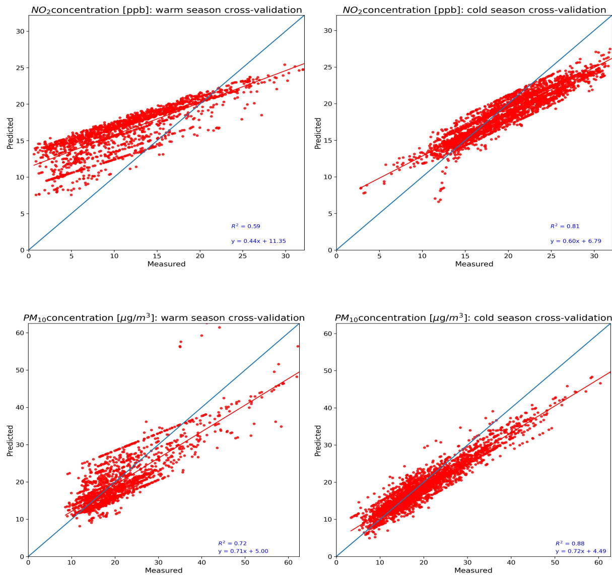
Figure 1. Cross-validation scatter plots of \text{NO}_2 (upper panel) and \text{PM}_{10} (lower panel) during warm (left panel) and cold (right panel) season
