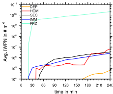
(f) PH: ice modes number
