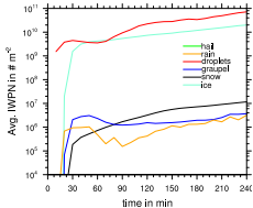
(c) HA: cloud number
