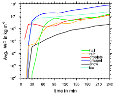
(a) HA: cloud mass
