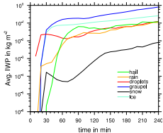
(b) REF: cloud mass
