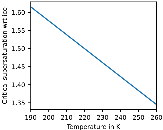
(a) Hom. nucleation threshold
