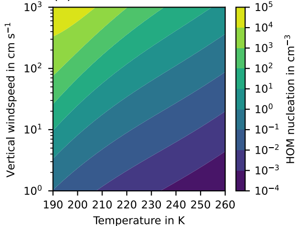
(b) Hom. nucleation event at SCR
