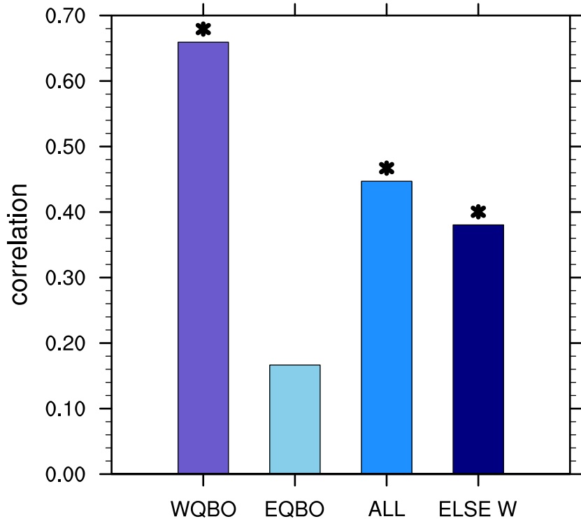
(a) correlation
