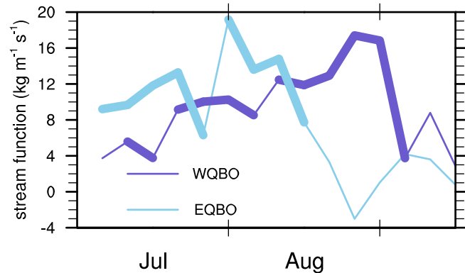
(c) difference in stream function
