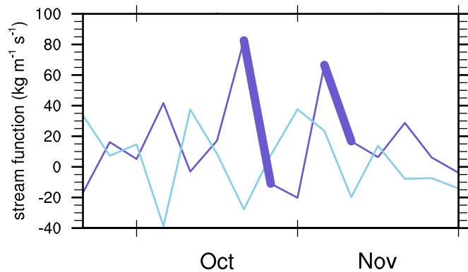
(c) difference in stream function
