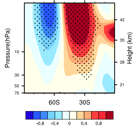
(c) U regression U August
