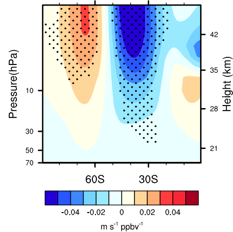
(f) O3 regression U August
