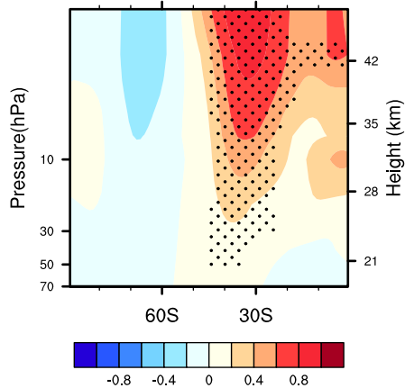
(a) U regression U June
