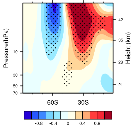
(b) U regression U July
