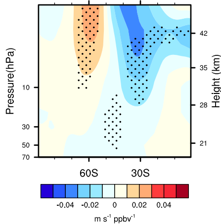
(e) O3 regression U July
