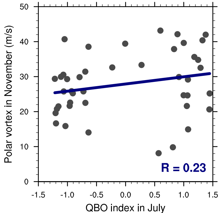
(b) QBO index & polar vortex
