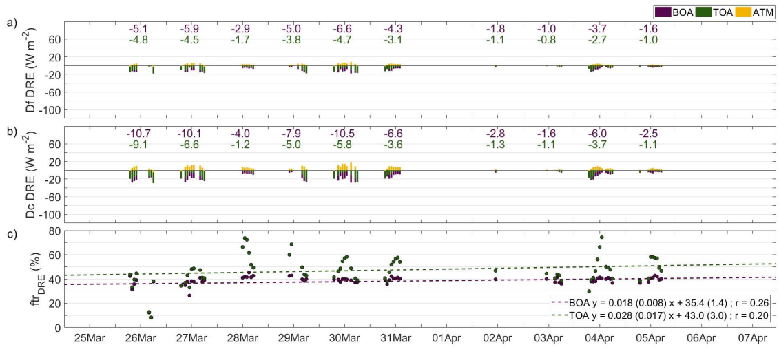
Figure S7. Same as Fig. S6, but at EVO station. A linear fit was calculated between 26 March and 5 April. Both linear fittings and correlation coefficients are included in the legend. The standard deviation of the slope and intercept are shown in brackets. The absolute increase in ftr DRE ratio ( \delta DRE ) of +0.018 \text{ \% h}^{-1} ( +0.028 \text{ \% h}^{-1} ) is equivalent to an increase of +0.77 \text{ \% day}^{-1} ( +0.64 \text{ \% day}^{-1} ) at BOA (TOA).
