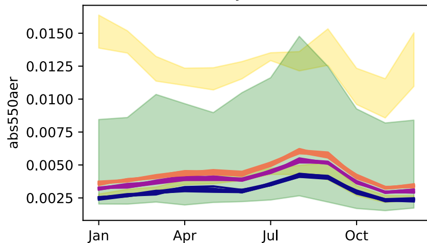
seasonal cycle: land-only
