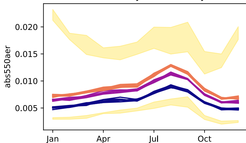
seasonal cycle: ocean-only
