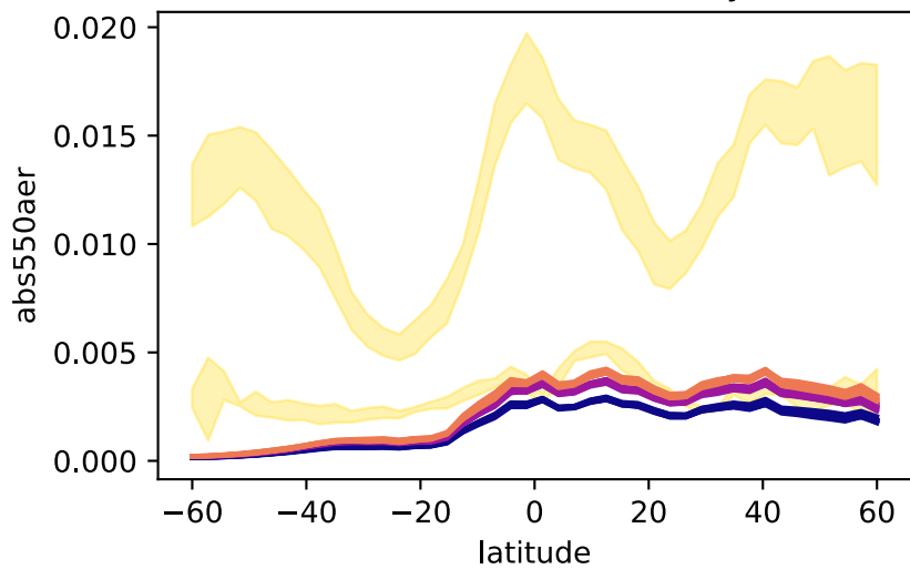
zonal mean: ocean-only
