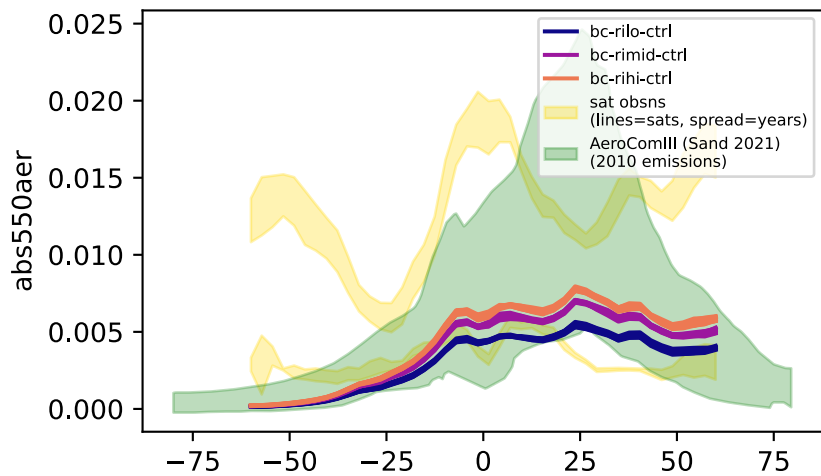
zonal mean: land-only
