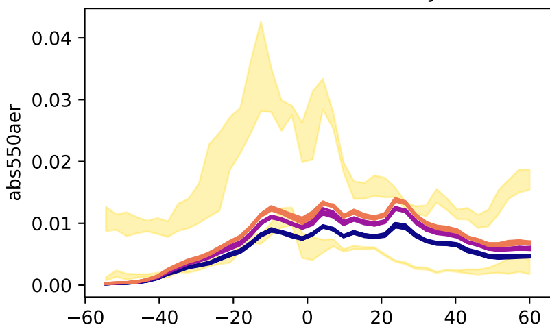
zonal mean: ocean-only
