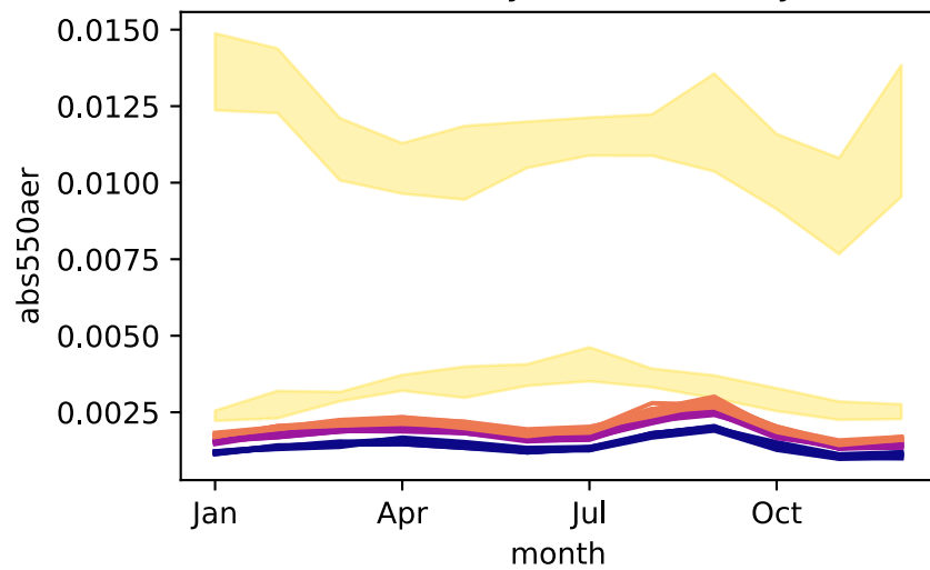
seasonal cycle: ocean-only
