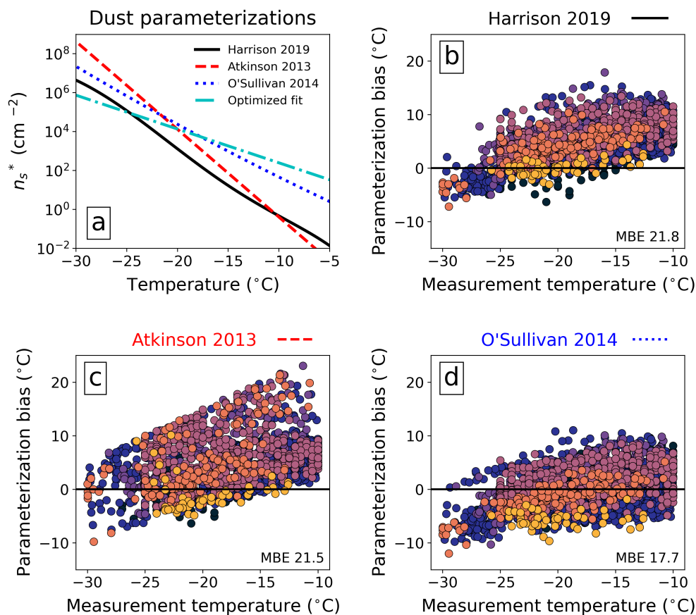
Figure S2. Sensitivity of simulated dust INP concentration to parameterizations of ice-nucleating activity. Same as Fig. 11 in manuscript but showing parameterization temperature bias. (a) temperature-dependent n_s curves of the three parameterizations, where n_s for the Harrison et al. (2019) and Atkinson et al. (2013) curves are scaled by 5% (accounting for dust K-feldspar content) to make all descriptions comparable. Panels (b), (c), and (d) show the parameterization temperature bias in the simulated N_{\text{INP}} as a function of measurement temperature in all regions for the Harrison et al. (2019), Atkinson et al. (2013), and O'Sullivan et al. (2014) parameterizations.
