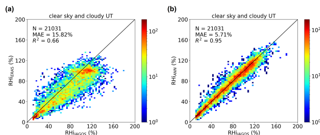
Figure 4. Distribution of (a) RH i ERA5 and (b) RH i ANN versus RH i AGOS in the UT in all-sky (clear and cloudy) conditions in the test data set. The number of data sets ( N ), the mean absolute error (MAE), and the coefficient of determination ( R^2 ) are shown in the panels.
