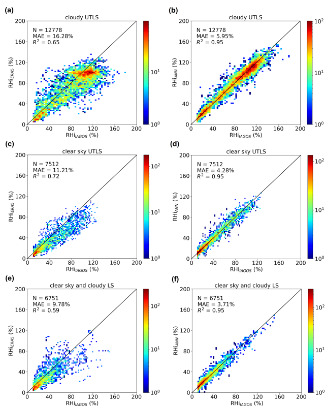
Figure 5. Comparison of \text{RH}_{\text{ERA5}} (left column) and \text{RH}_{\text{ANN}} (right column) against \text{RH}_{\text{IAGOS}} in the (a, b) cloudy UTLS, (c, d) clear-sky UTLS, and (e, f) clear-sky and cloudy (or all-sky) LS regions in the test data set. The number of data sets ( N ), the mean absolute error (MAE), and the coefficient of determination ( R^2 ) are indicated in the individual panels.
