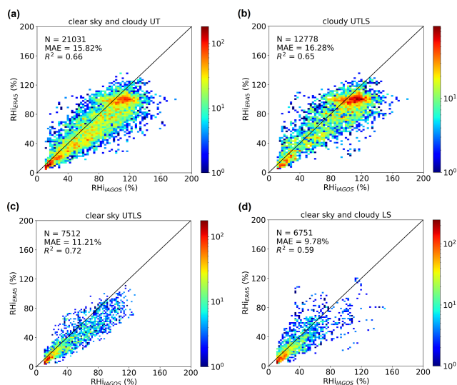
Figure 2. Comparisons of \text{RHi}_{\text{ERA5}} against \text{RHi}_{\text{IAGOS}} in (a) clear-sky and cloudy UT, (b) cloudy UTLS, (c) clear-sky UTLS, and (d) clear-sky and cloudy LS in the test data set between 200 and 400 hPa over the Atlantic, Europe, and Africa for the year 2020.
