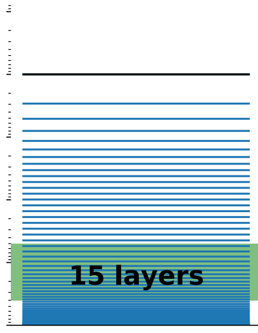
MOZART-3
