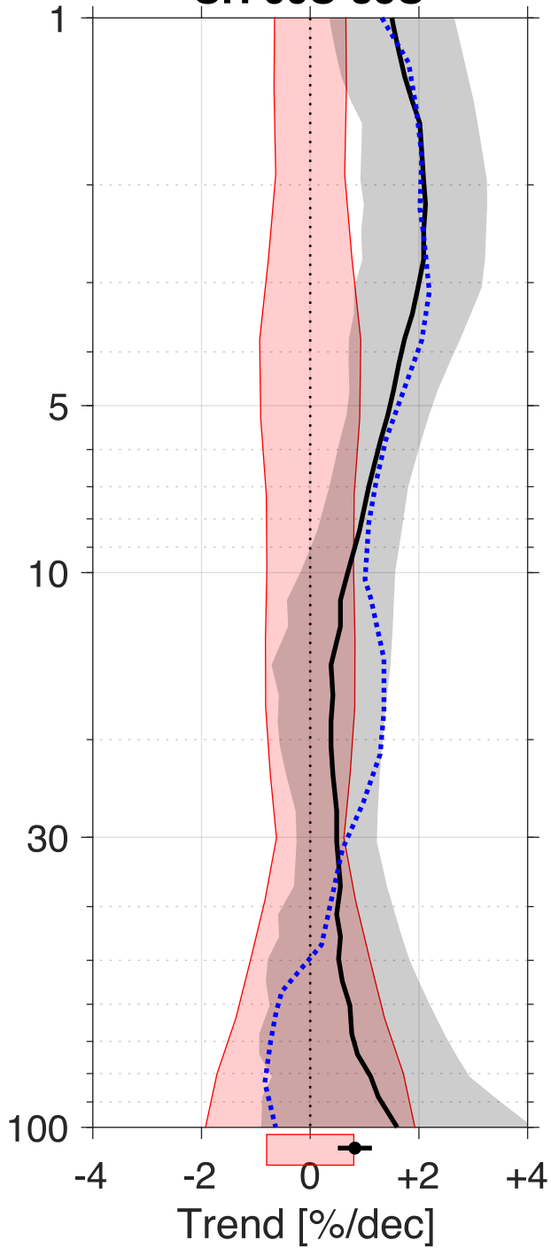
SH 60S-35S
