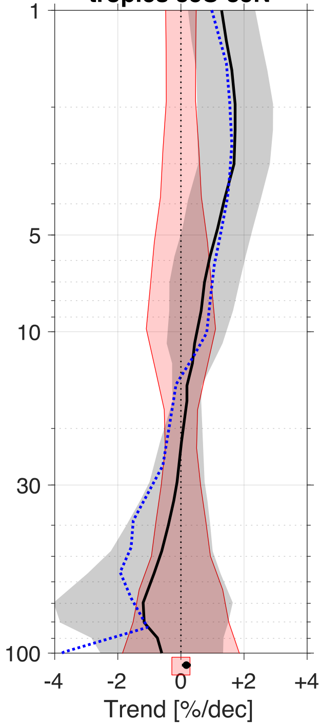
tropics 35S-35N
