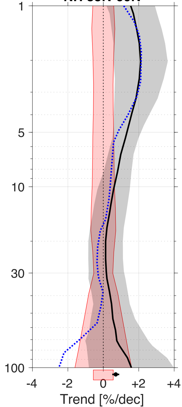
NH 35N-60N
