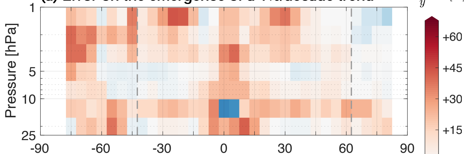
(b) Error on the emergence of CCMI1 trends
