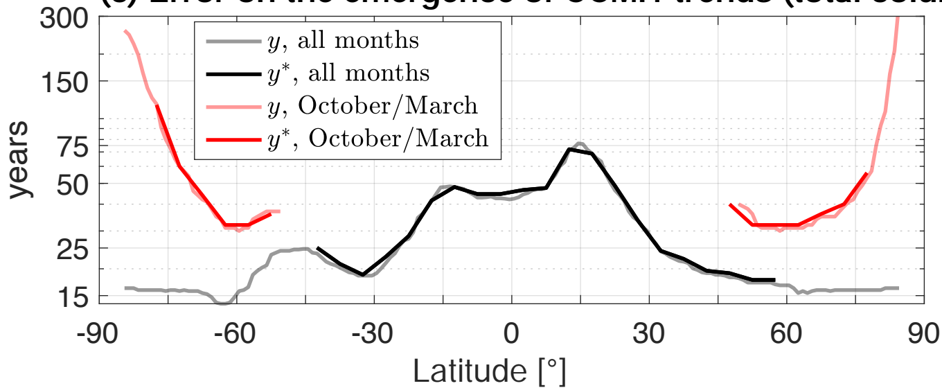
(c) Error on the emergence of CCMI1 trends (total column)
