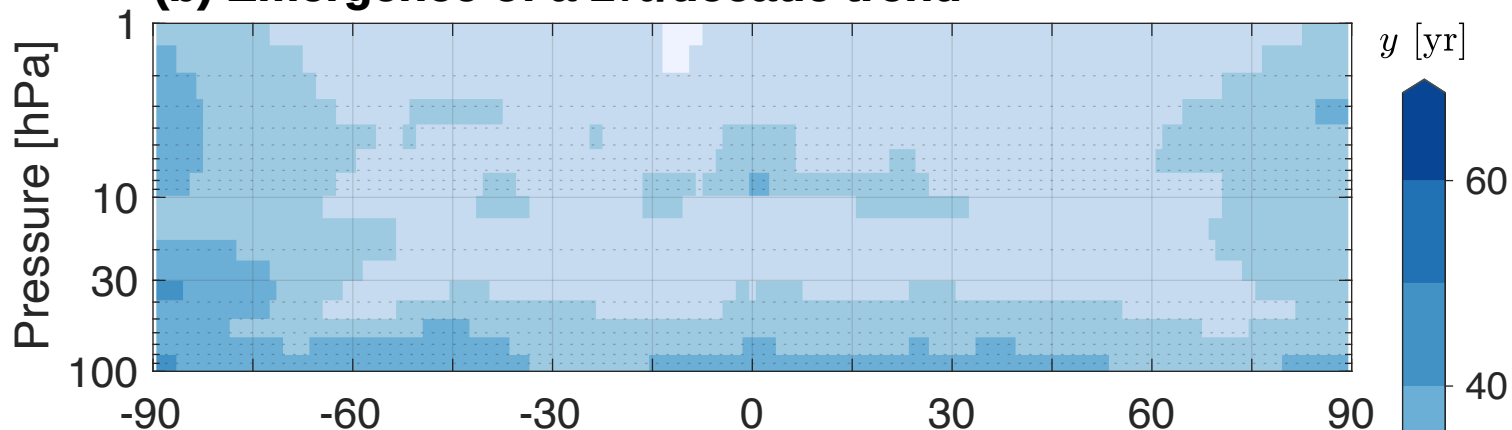
(c) Emergence of CCMI1 trends
