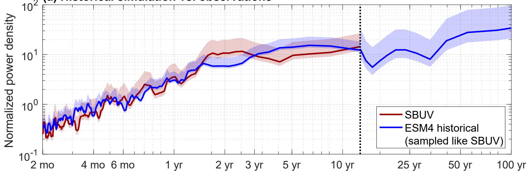
(a) Historical simulation vs. observations
