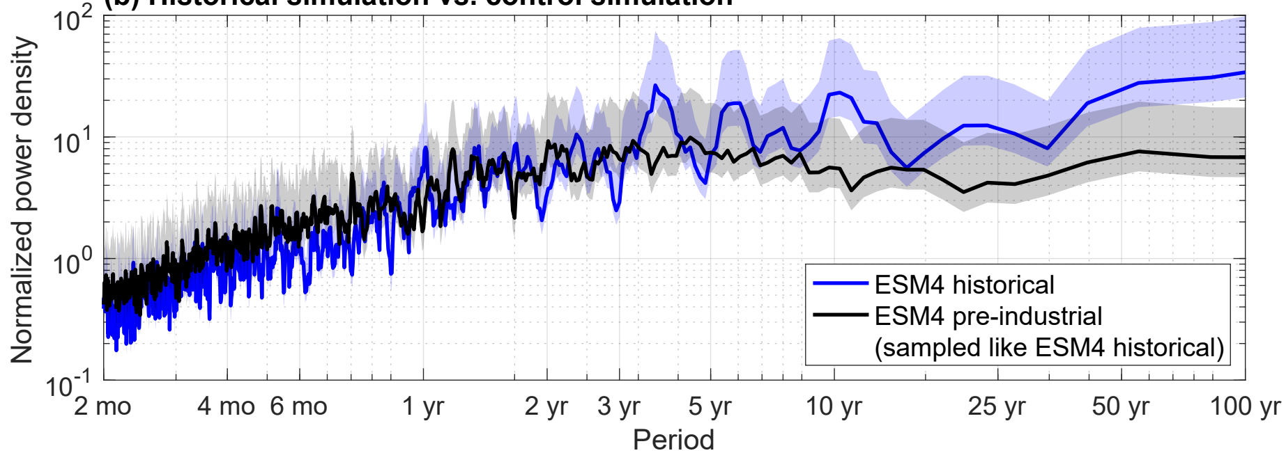
(b) Historical simulation vs. control simulation
