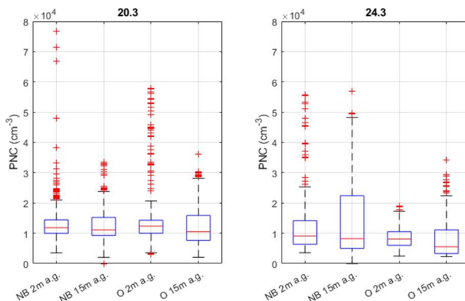
Figure 7. Boxplots of PNC measured with a drone in the open area (O 2 m a.g., O 15 m a.g.) and behind the noise barrier (NB 2 m a.g., NB 15 m a.g.) separately for 20 and 24 March. The median values are indicated with horizontal red lines, the blue box resembles the lower and upper 25th and 75th percentiles, the whiskers represent the lowest and highest values considered for data evaluation, and the outliers are marked with red plus marks. The a.g. stands for above ground.
