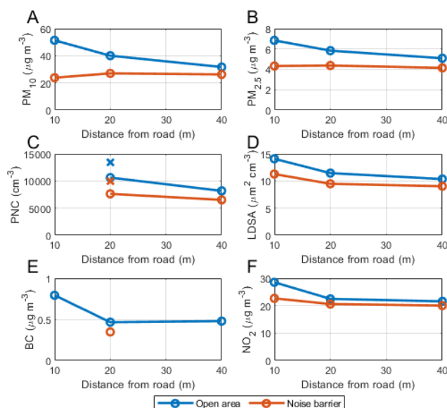
Figure 5. (A) \text{PM}_{10} , (B) \text{PM}_{2.5} , (C) PNC, (D) LDSA, (E) BC, and (F) \text{NO}_2 gradients in the open area and behind the noise barrier. In panel (C), the PNC gradient has been measured with AQ urban sensors, and PNCs measured with CPCs have been presented with “X”. In panel (E), the concentrations at 20 m have been measured with AE51 and concentrations at 10 and 40 m with ObservAir sensors. The gradients have been calculated over all the measured data. The data coverages for each parameter are presented in Supplement Table S1.
