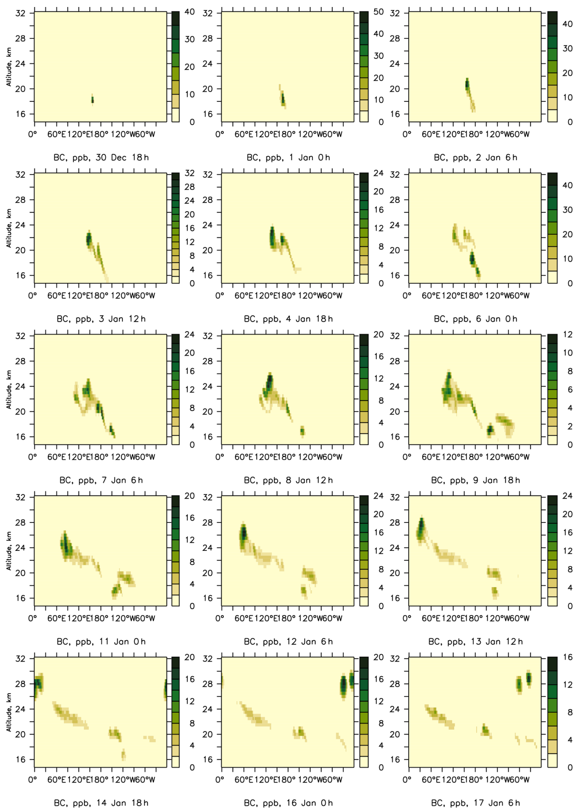
Figure A8. Simulated BC in lofting vortices at 35° S against altitude in km, every 30 h, beginning on 30 December 2019.
