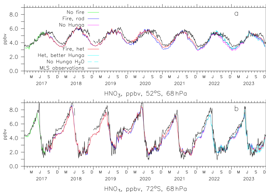
Figure 6. Simulated and observed HNO 3 at 68 hPa at 52° S (a) and 72° S (b). EMAC scenarios of Table 2 see legend.
