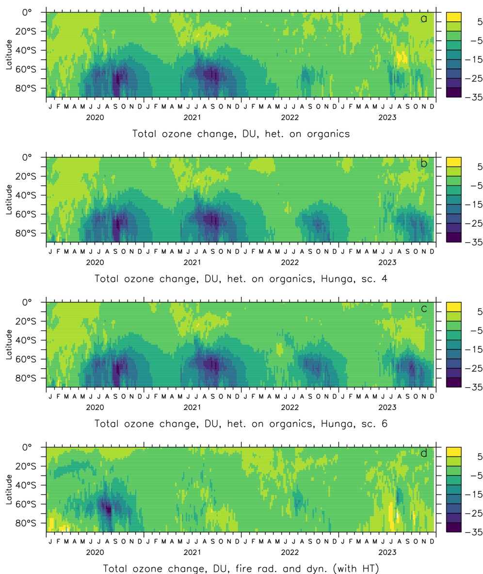
Figure 8. Calculated total ozone change from heterogeneous chlorine activation on organics from fires ( a , scenario 4 against scenario 2) and additionally the eruption of Hunga (scenario 4, b , and scenario 6, c , against scenario 3). The lower panel ( d ) shows the radiative/dynamical effects of fires (scenario 2 against scenario 1, in 2023 mostly noise).
