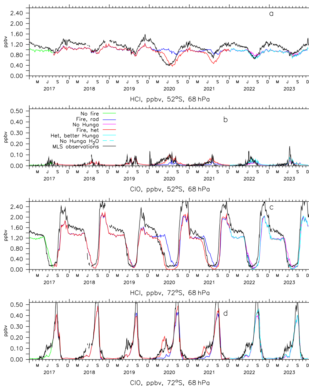
Figure 4. Simulated and observed HCl at 68 hPa at 52° S (a) and 72° S (c). Calculated and observed ClO in panels (b) and (d). Colors in the legend indicate the EMAC scenarios of Table 2. 5 d averages for EMAC, daily averages with 5 d boxcar smoothing for MLS.
