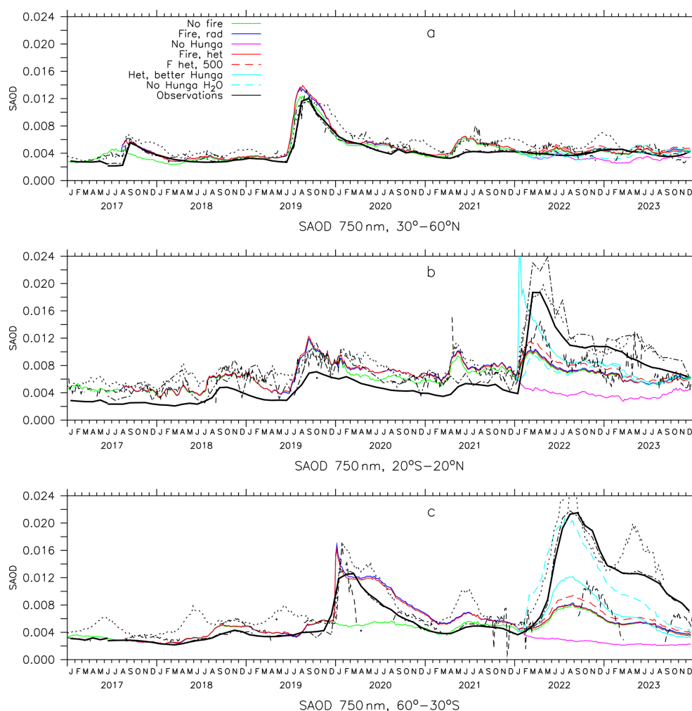
Figure 1. Stratospheric aerosol optical depth in tropical latitudes (b), northern (a) and southern midlatitudes (c), zonal averages. Colors: EMAC simulations of legend and Table 2. Black thick: GloSSAC V2.22, after June 2017 observations by SAGE III/ISS, cloud cleared, black dash-dotted: GloSSAC V2.22, SAGE III/ISS, all, black dotted: observed by OMPS-LP, black dashed: observed by OSIRIS. GloSSAC monthly averages, all other curves 5 d averages.
