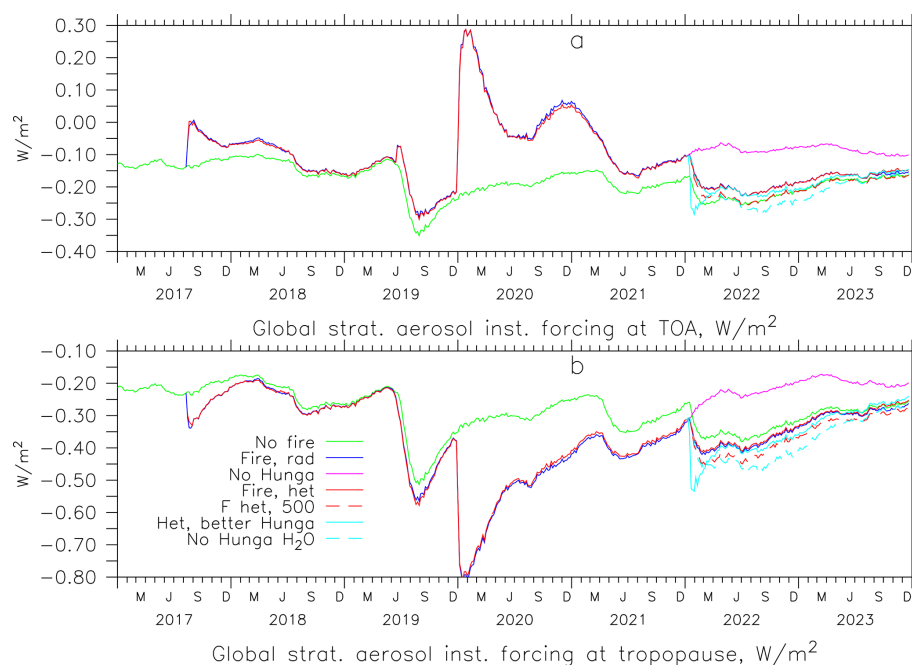
Figure 2. Calculated instantaneous radiative forcing by aerosol at the Top of the Atmosphere (TOA, a ) and tropopause altitude ( b ). Colors of EMAC simulations see legend and Table 2.
