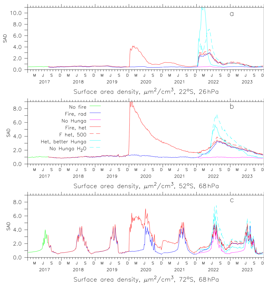
Figure 3. Calculated surface area density ( \mu\text{m}^2 \text{cm}^{-3} ) for heterogeneous chemistry in the middle stratosphere in southern subtropics (a) and the lower stratosphere in southern middle (b) and high (c) latitudes. Colors see legend and Table 2. The green curve is shown only for 2017 since very close to the blue one later.
