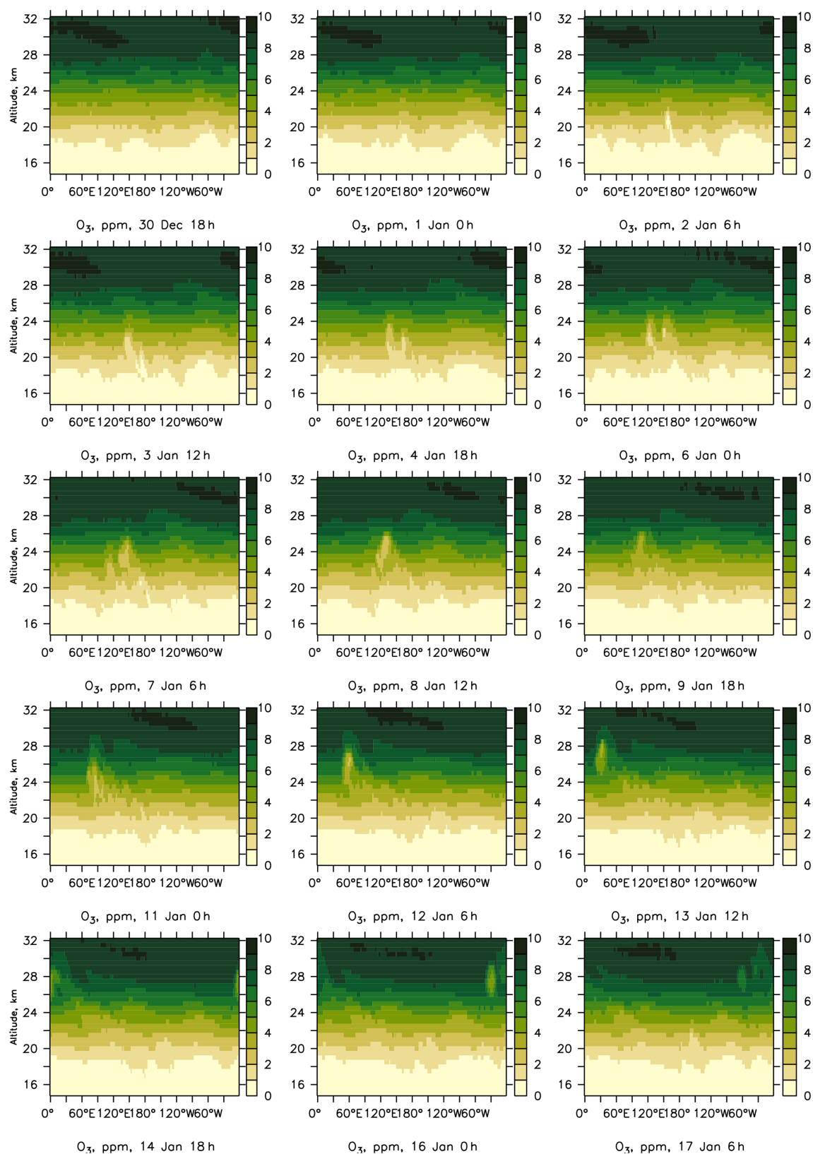
Figure A9. Simulated depleted ozone in the vortices of Fig. A8.
