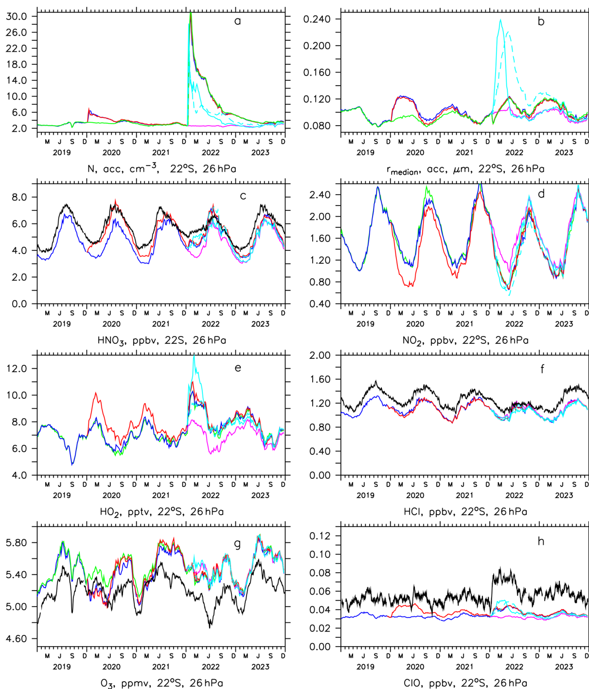
Figure A10. Number concentration, median radius (accumulation mode) and chemistry at latitude and altitude of the Hunga injection, colors see Table 2 and Fig. A1. MLS ClO observations are shown with 15 d boxcar smoothing.
