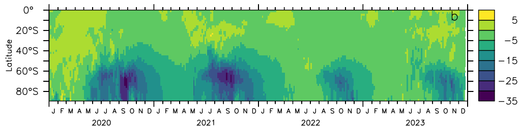
Total ozone change, DU, het. on organics, Hunga, sc. 4
