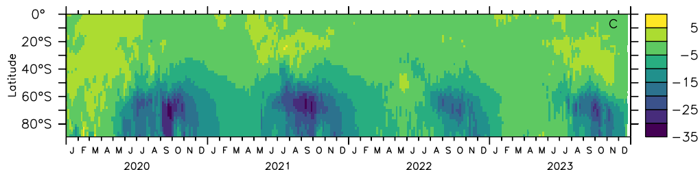
Total ozone change, DU, het. on organics, Hunga, sc. 6
