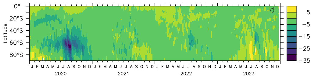
Total ozone change, DU, fire rad. and dyn. (with HT)
