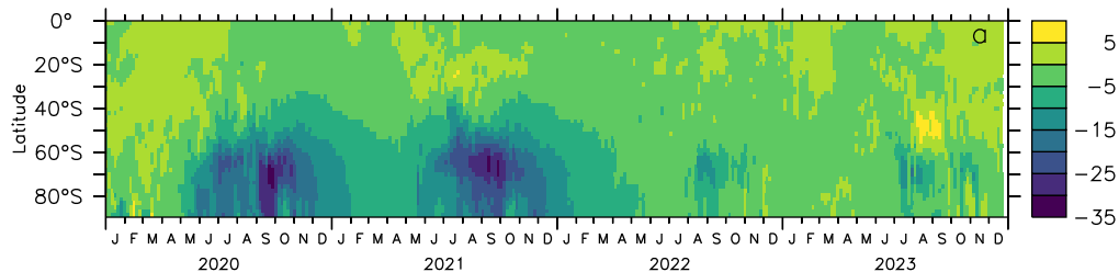
Total ozone change, DU, het. on organics
