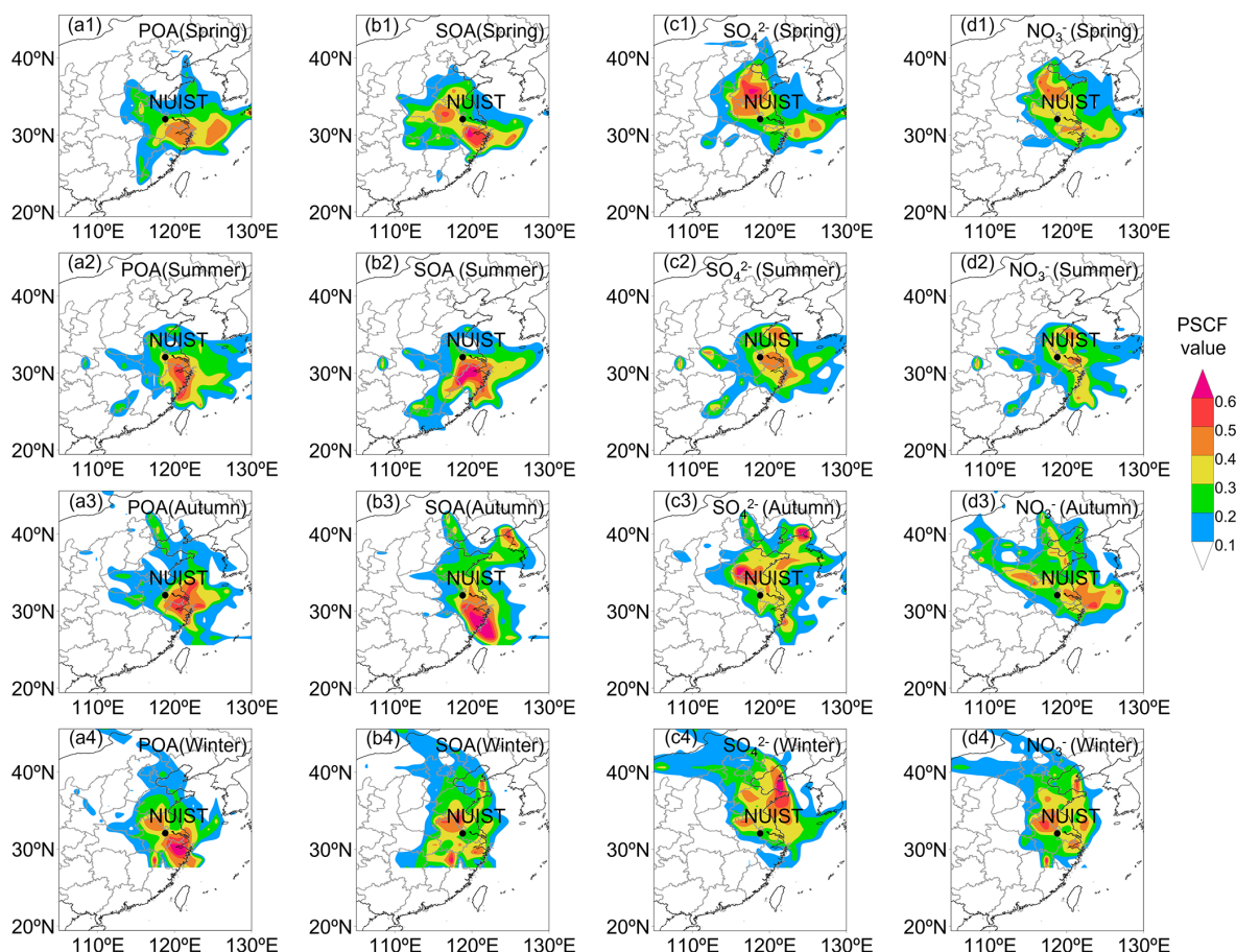
Figure 9. PSCF analysis of (a) POA, (b) SOA, (c) sulfate, and (d) nitrate in \text{PM}_{2.5} during four seasons. The black dot indicates the NUIST site. The color scale indicates the values of PSCF.
