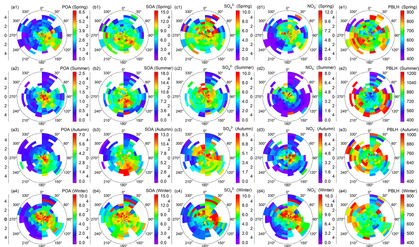
Figure 10. Pollution roses of (a) POA, (b) SOA, (c) sulfate, (d) nitrate and (e) PBLH during four seasons. The data are grouped into grids with increments of WS and WD being 0.5 \text{ m s}^{-1} and 20^\circ , respectively. The unit of color scale is \mu\text{g m}^{-3} .
