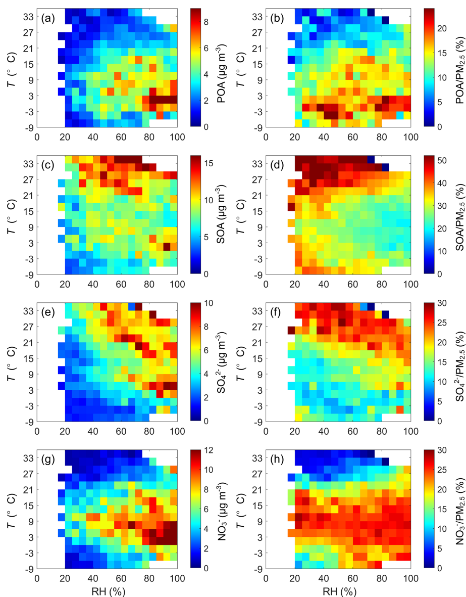
Figure 3. RH/ T dependence of mass concentrations and mass fractions in \text{PM}_{2.5} of POA, SOA, sulfate, and nitrate for the entire period. The data are grouped into grids with increments of RH and T being 5 % and 3 °C, respectively. Grid cells with the number of data points fewer than 10 are excluded.
