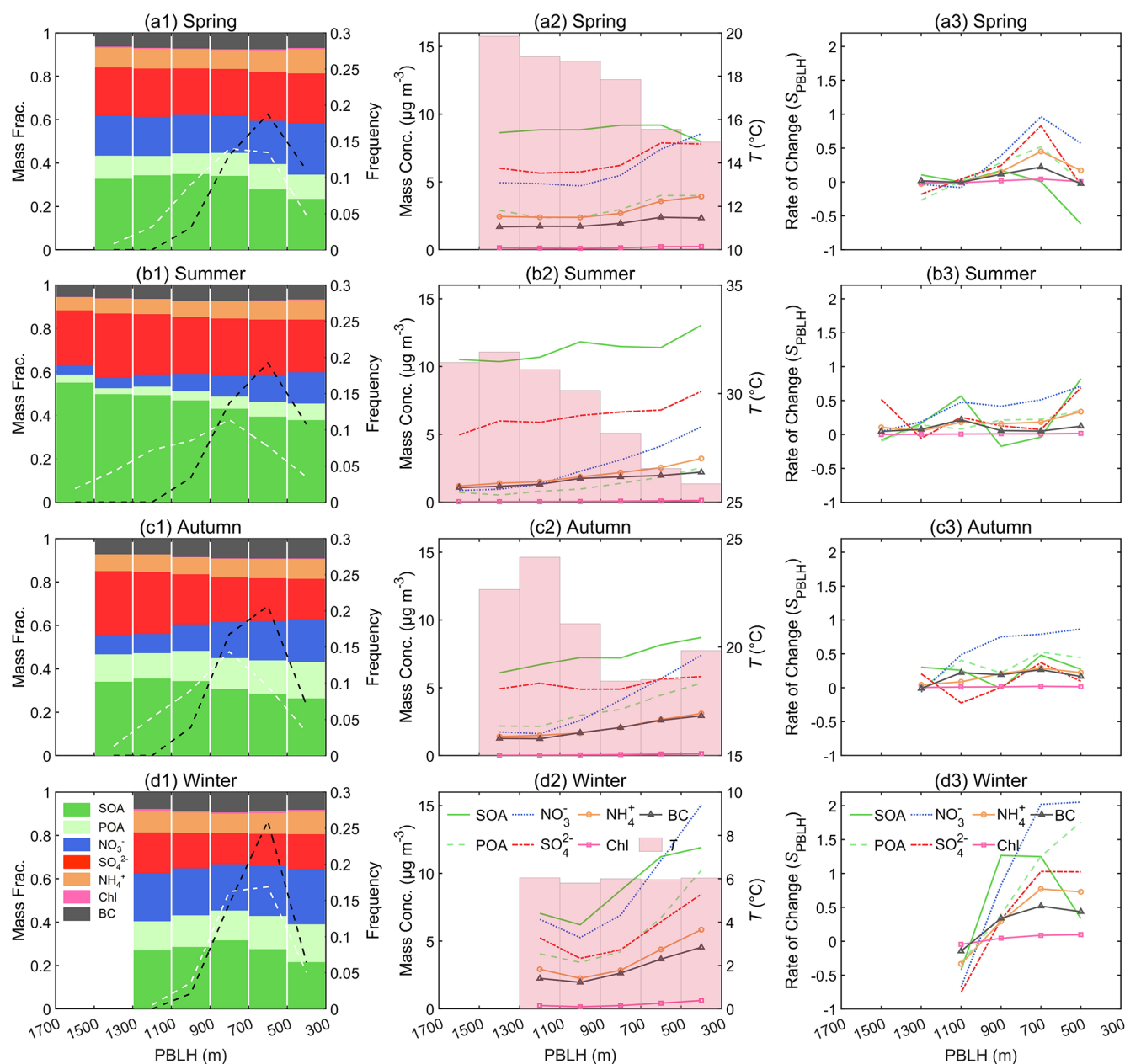
Figure 8. (a1–d1) The mass fraction of \text{PM}_{2.5} chemical components as a function of PBLH distribution (left y axis) and frequency distribution of PBLH data points relative to the total number of data points (right y axis, white dashed line represents daytime and black dashed line represents nighttime) in four seasons. (a2–d2) The mass concentration of \text{PM}_{2.5} chemical components (left y axis) and the T (right y axis, pink columns) as a function of PBLH distribution in four seasons. (a3–d3) The rate of change in \text{PM}_{2.5} chemical components ( S , units: \mu\text{g m}^{-3} (100\text{ m})^{-1} ) with the decrease of PBLH in four seasons. The data are grouped in PBLH bins with 200 m increments. Bins with the number of data points fewer than 10 are excluded.
