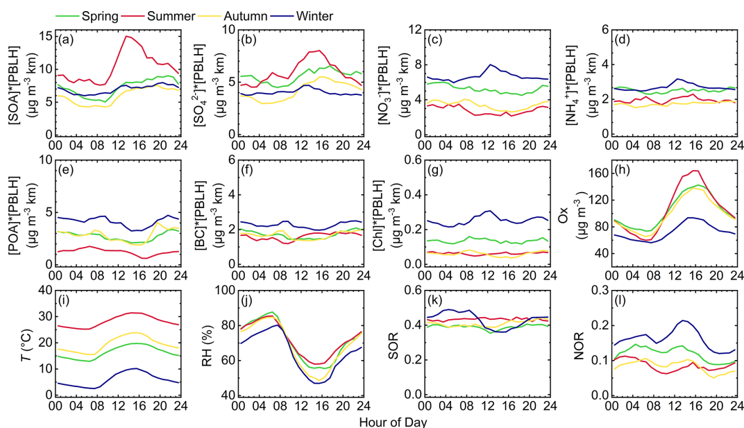
Figure 7. Average diurnal variations of (a–g) PM 2.5 chemical components after removing the dilution effect of planetary boundary layer, (h) photochemical oxidant (O x ), (i) T, (j) RH, (k) sulfate oxidation ratio (SOR), and (l) nitrogen oxidation ratio (NOR) during four seasons. To isolate emission sources and secondary formation effects on local pollution, the average diurnal variations of PM 2.5 chemical components are multiplied by PBLH to remove the dilution effect (denoted as [component]*[PBLH], e.g., [POA]*[PBLH], [BC]*[PBLH]) in a–g panels.
