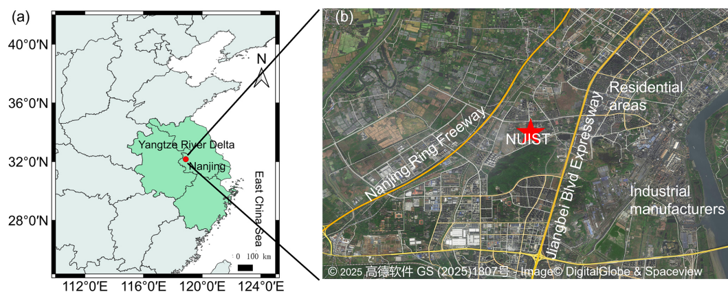
Figure 1. (a) Geographical location of Nanjing in the Yangtze River Delta and (b) the distribution of pollution sources around the NUIST observation site (source: Gaode Map, GS (2025)1807). The base map contains data from DigitalGlobe and Spaceview.
