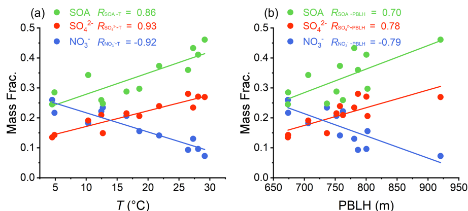
Figure 4. The correlation and linear fitting lines between the monthly average mass fractions of SOA, sulfate, nitrate in PM 2.5 and the corresponding monthly average (a) T and (b) PBLH. R_{\text{SOA}-T} , R_{\text{SO}_4^{2-}-T} , R_{\text{NO}_3^-}-T : correlation coefficients with T . R_{\text{SOA}-\text{PBLH}} , R_{\text{SO}_4^{2-}-\text{PBLH}} , R_{\text{NO}_3^-}-\text{PBLH} : correlation coefficients with PBLH.
