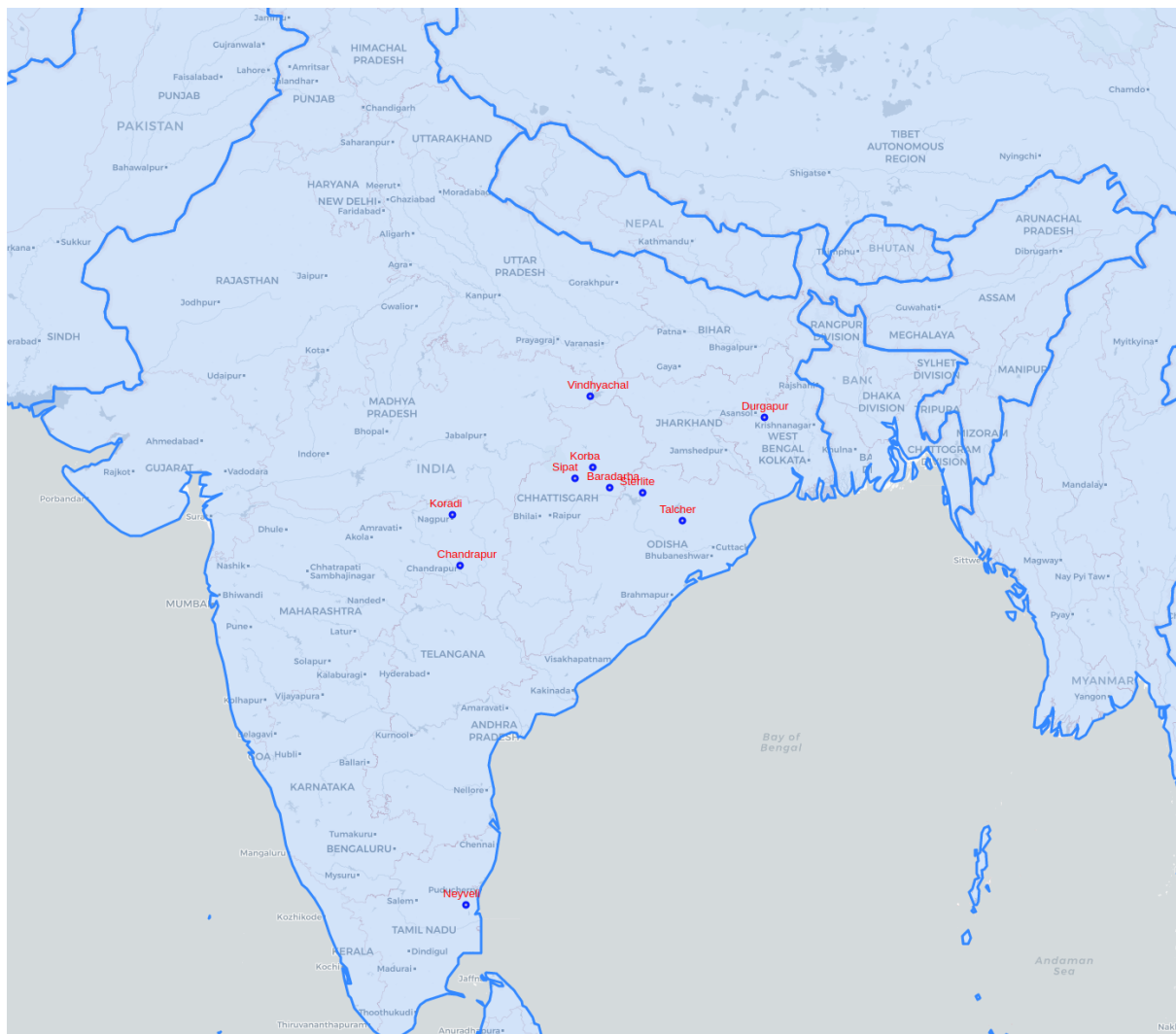
Figure S9. The locations of top 10 of highest emission sources in our inventory, © Google Maps, 2024.
