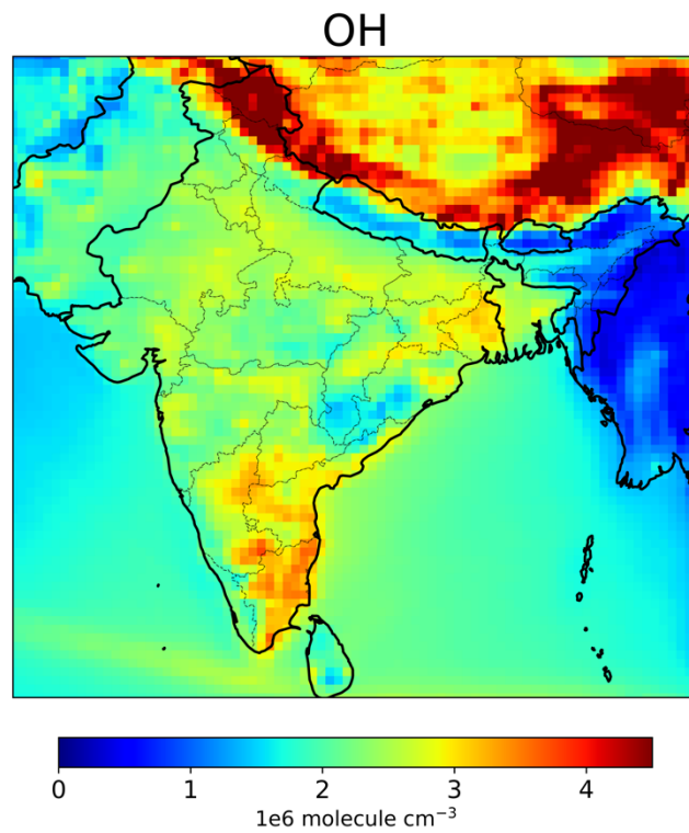
Figure S10. Annual mean OH concentration from CAMS simulation averaged from 2019 to 2023.
