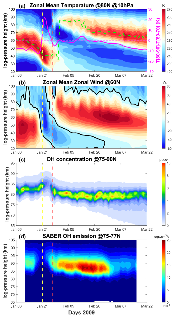
Figure 1. Time versus log-pressure height cross-section of SD-WACCM-X zonal-mean (a) temperature at 80^\circ N, (b) zonal wind at 60^\circ N, (c) OH concentration, and SABER (d) OH emission, during 6 January–22 March 2009. The solid pink line represents the meridional temperature difference between 60\sim 70 and 80\sim 90^\circ N ( T[80\sim 90^\circ] - T[60\sim 70^\circ] ), and the dashed green line is the stratopause height. The black solid contour in panel (b) denotes the zero-wind line. Vertical dashed yellow and red lines are the onset of the stratosphere warming stage and elevated stratopause stage, respectively.
