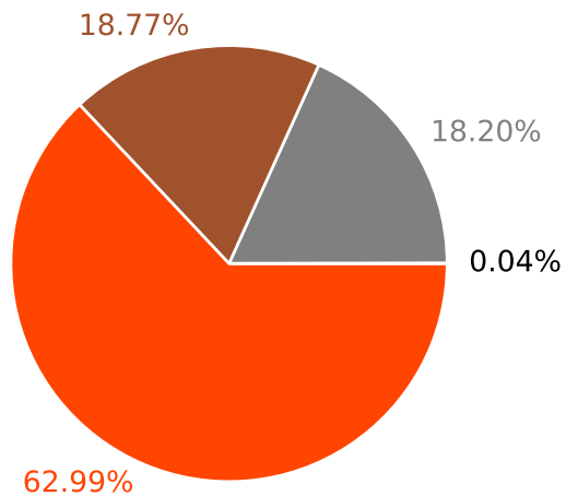
(a) - REF
