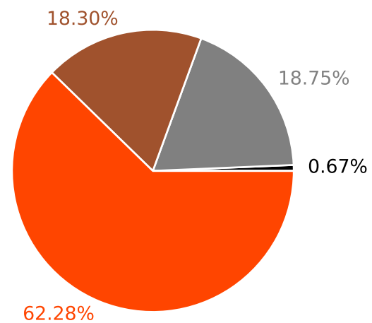
(f) - RIGHI21
